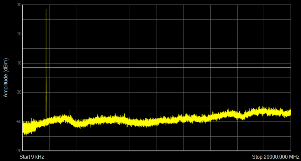
Band66 16QAM BW=5MHz Channel=132647 RB Size=1 Position=#0
