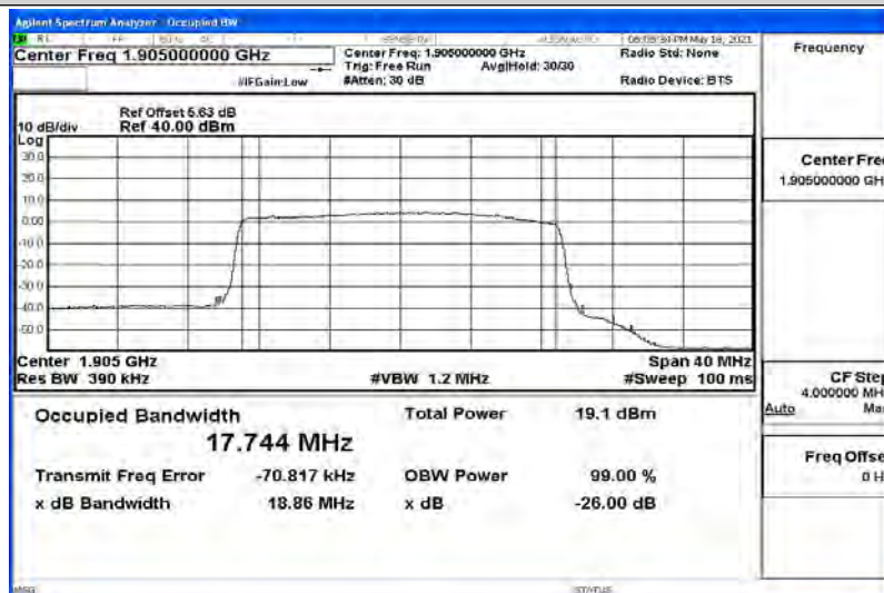
Band25-20MHz-16QAM-26590-100RB#0-17.744
