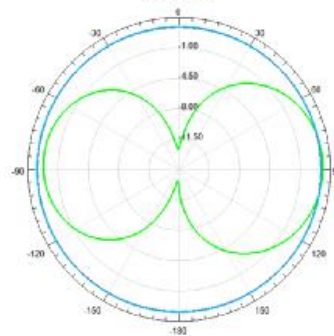
Gain Plot 2
