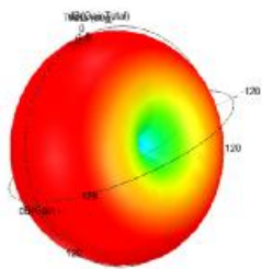
Gain Plot 1
