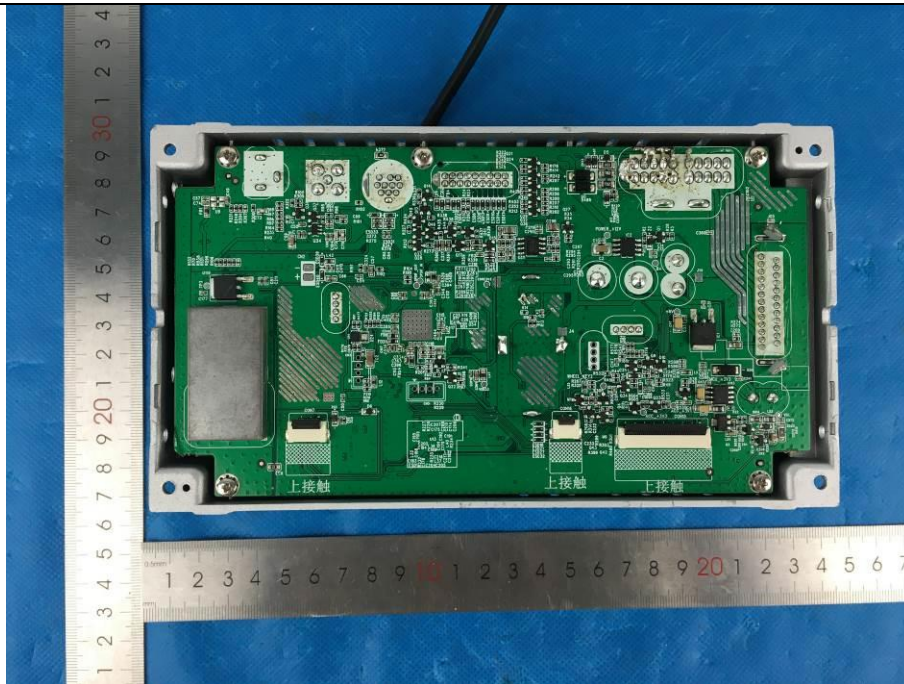
Photo 1 (For model CAR710W)
