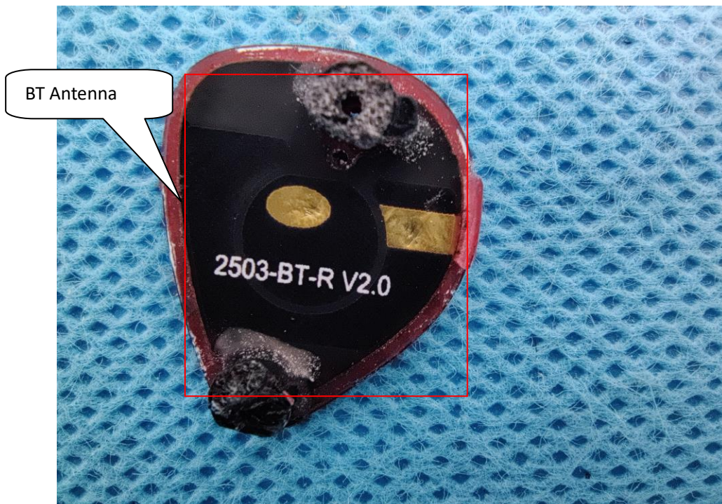
INTERNAL VIEW OF EUT - Right Earphone (FIGURE 4)
