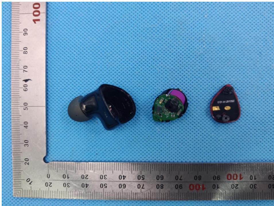
OPEN VIEW OF EUT - Right Earphone
