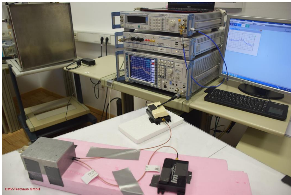
Picture 9: Relative conducted measurements with tag
