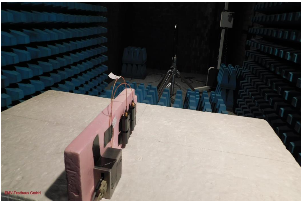
Picture 4: CDC, radiated emission test 9 kHz -30 MHz – position Z (front view)
