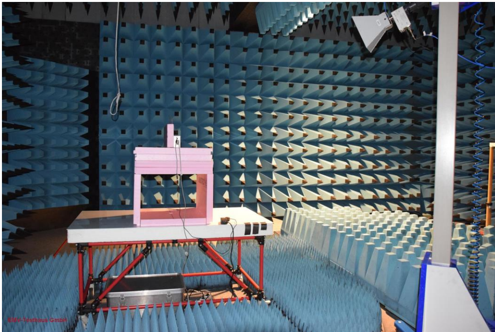
Picture 7: AC, radiated emission test 1 GHz – 10 GHz – position Z (front view)
