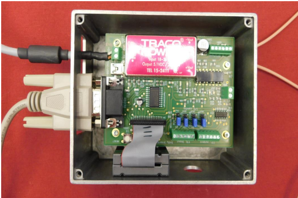
Picture 1: Top view of opened EUT
