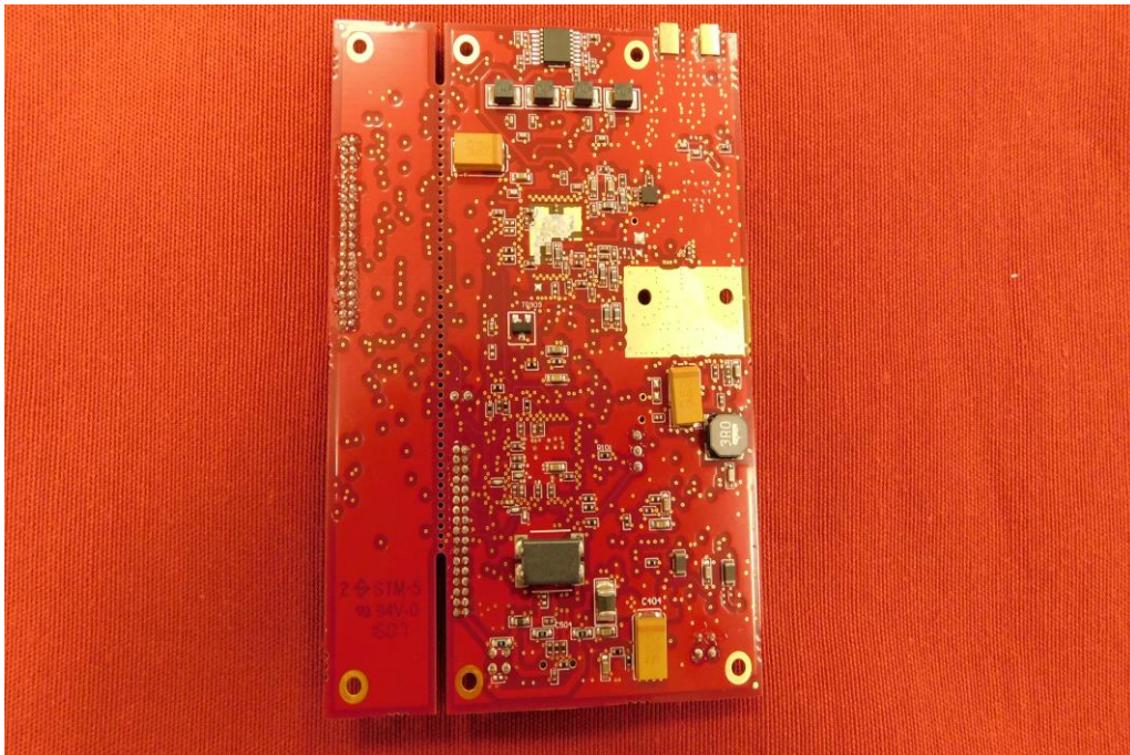
Picture 9: RF module with antenna connectors – back view
