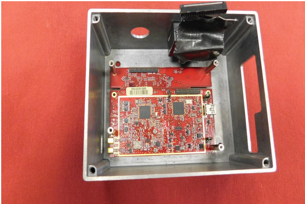
Picture 3: RF module with antenna connectors in housing without ribbon cable – top view
