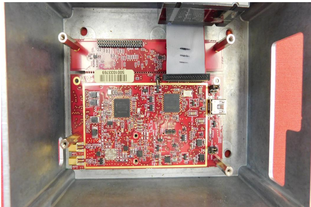
Picture 2: RF module with antenna connectors in housing – top view
