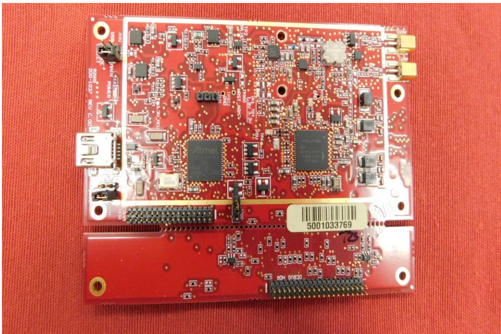
Picture 8: RF module with antenna connectors – top view
