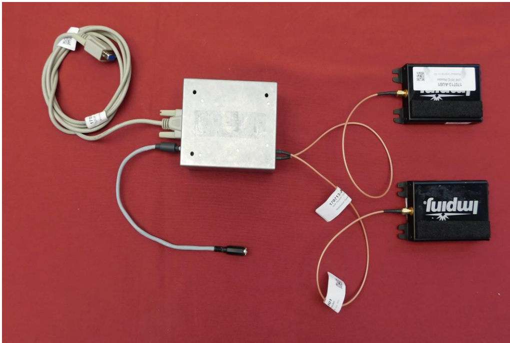
Picture 3: Top view of EUT with antennas
