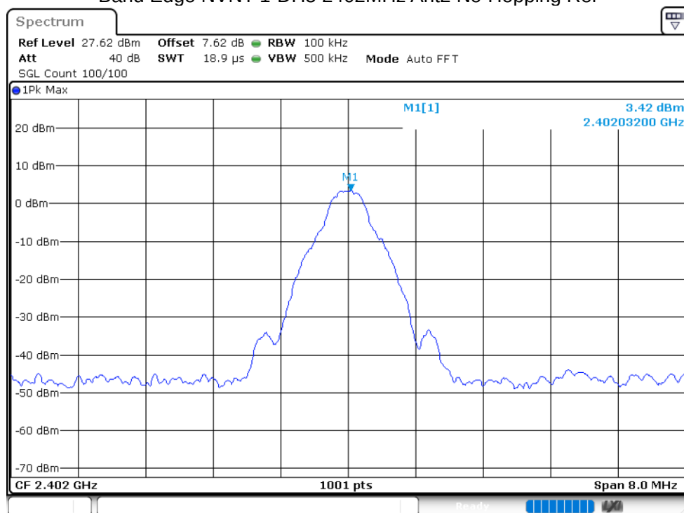
Band Edge NVNT 1-DH5 2402MHz Ant2 No-Hopping Ref
