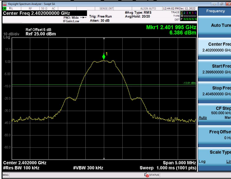
2_Bandedge_BLE_1Mbps_2402
