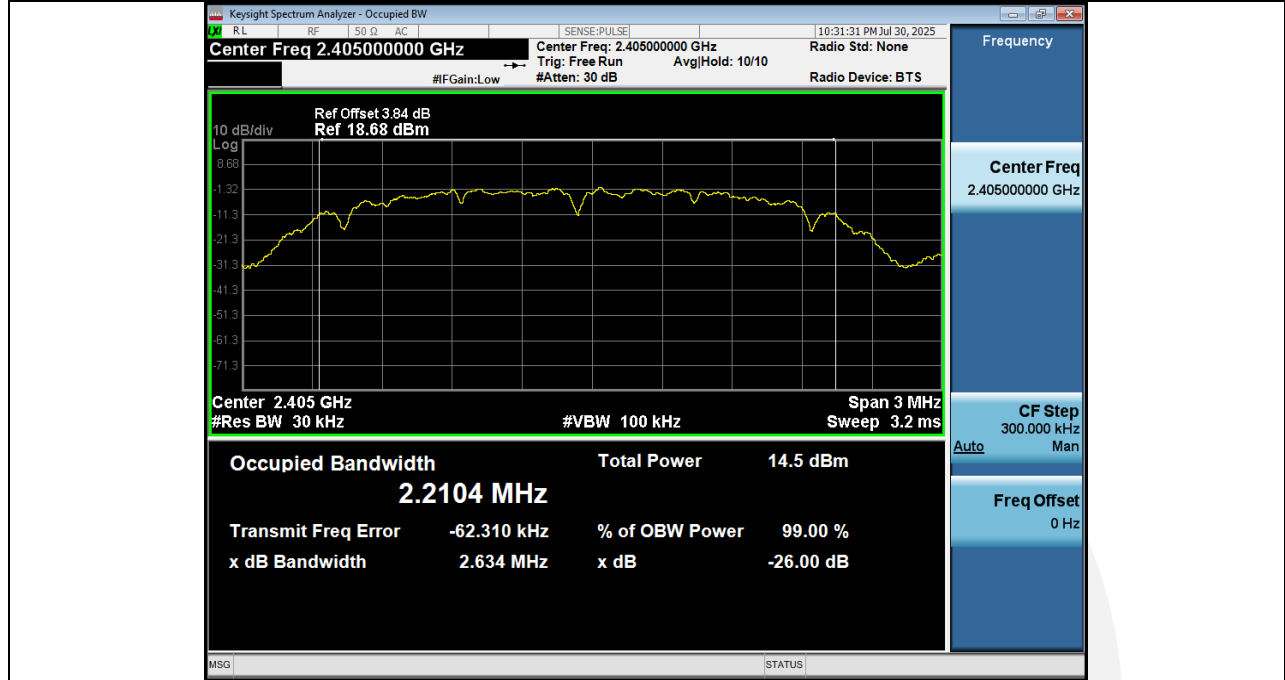
99% Occupied Bandwidth NVNT ANT1 250kbps 2405
