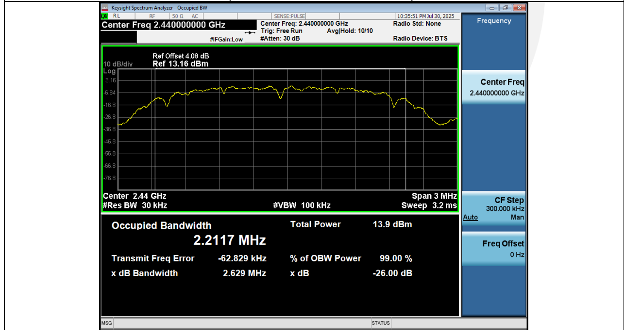
99% Occupied Bandwidth NVNT ANT1 250kbps 2440
