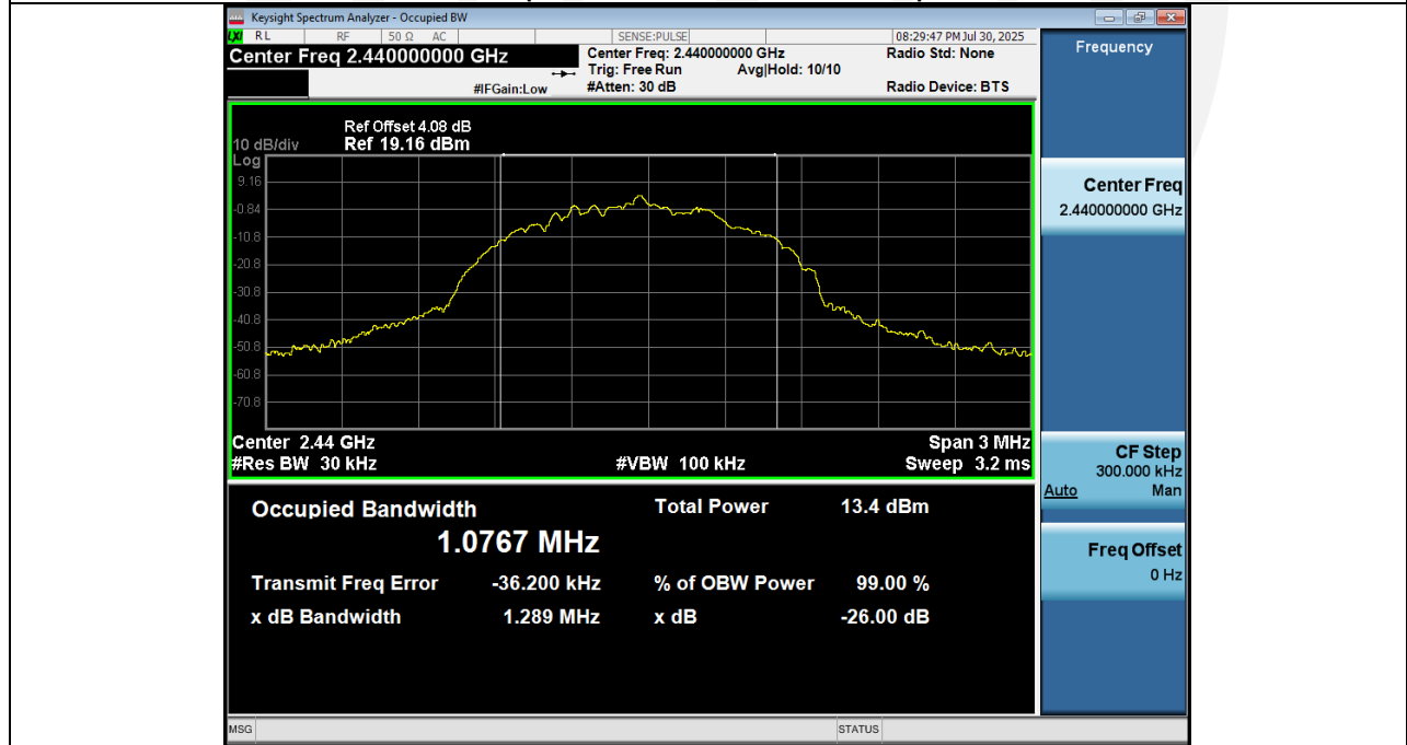
99% Occupied Bandwidth NVNT ANT1 1Mbps 2440
