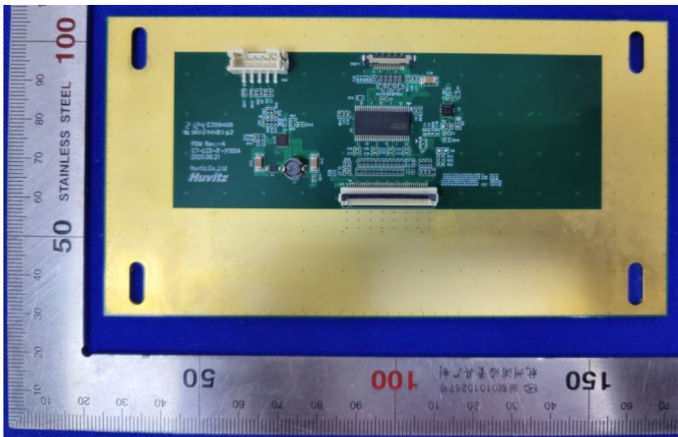
LCD sub board
