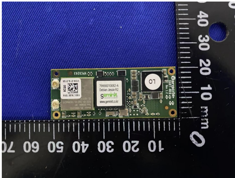
Radio module front (remove shielding)
