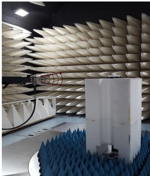
Figure B5. Radiated Setup- High Range
