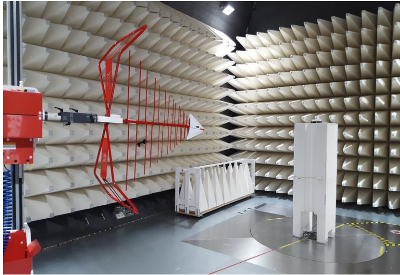
Figure B4. Radiated Setup – Low Range
