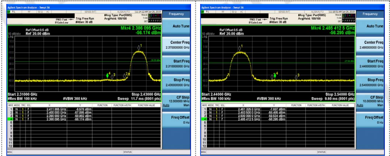
Left bandedge
