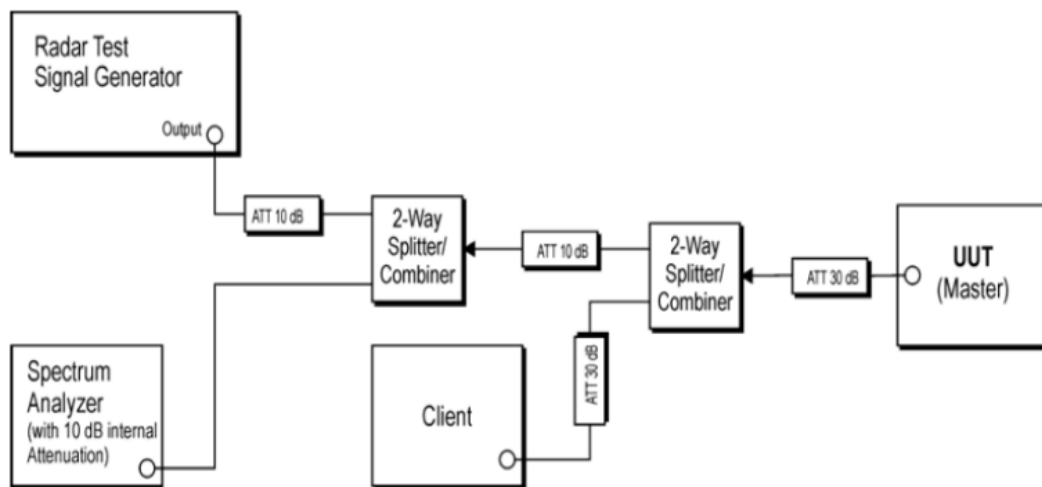
Figure 7-1. Test Setup
