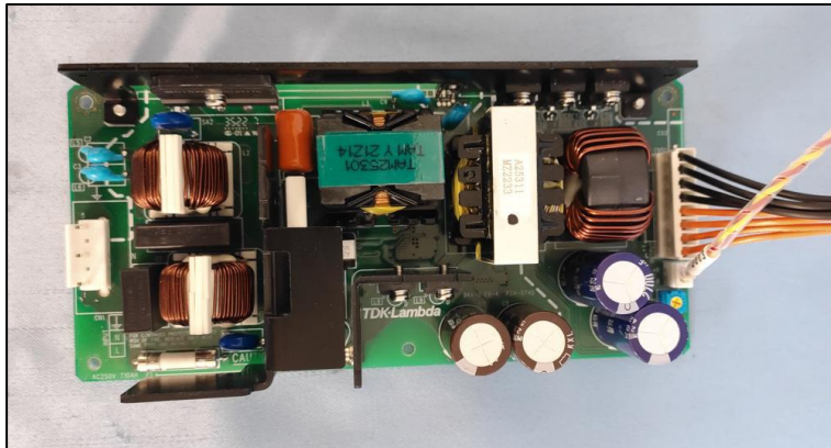
TDK Lambda power supply 24 VDC output
