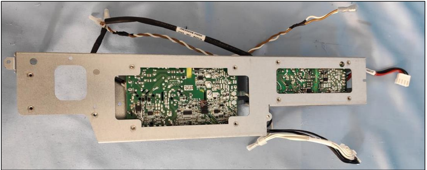
Power Supply Unit assembly
