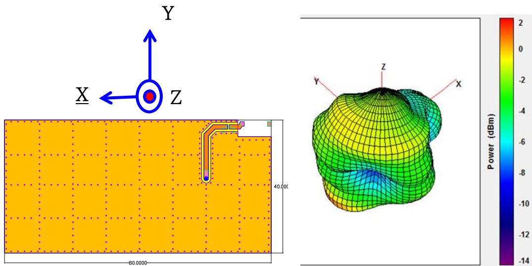
Radiation Pattern
