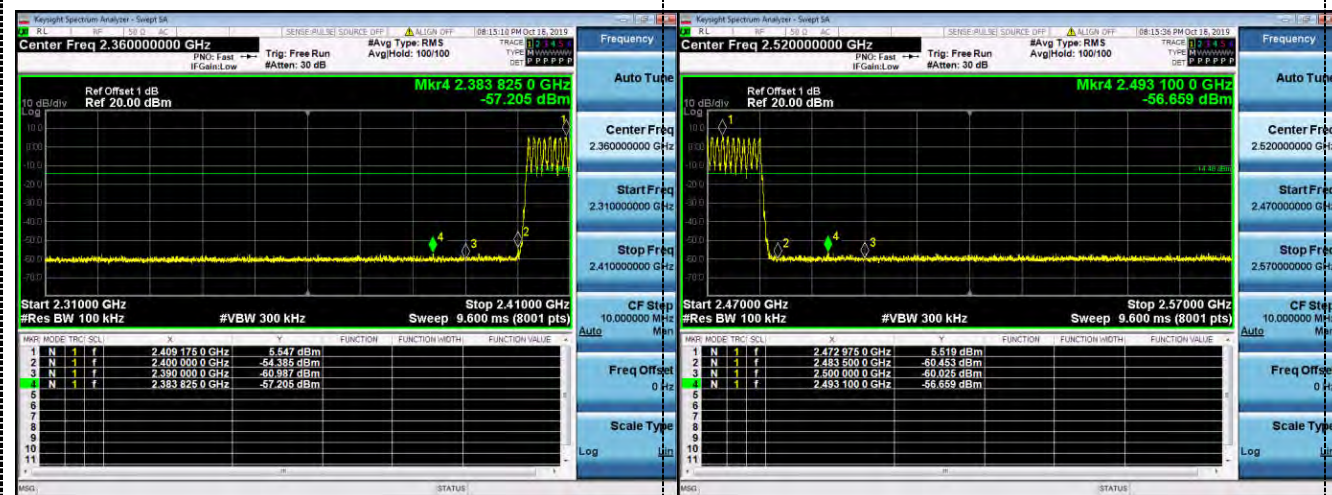
Left Band edge hoping on
