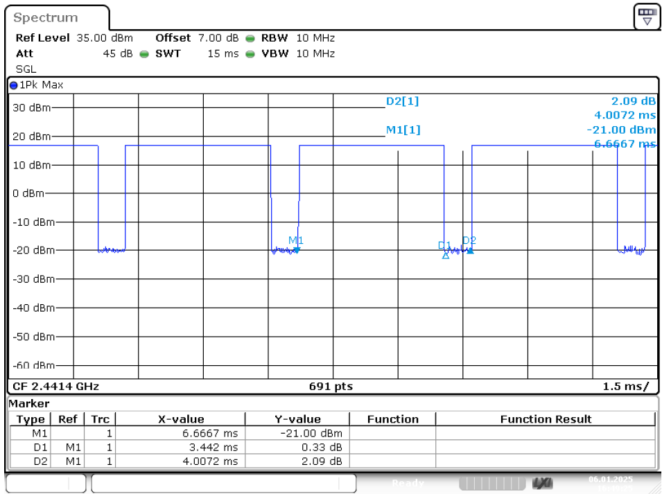
Duty Cycle
