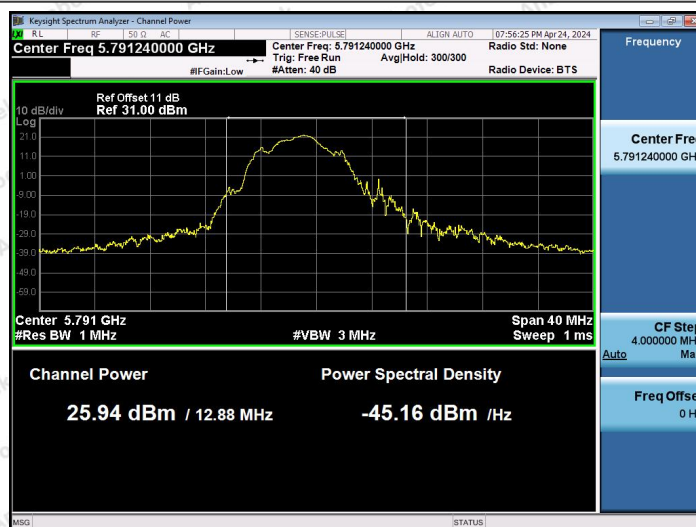
5.8G-Ant1-5790-PASS
