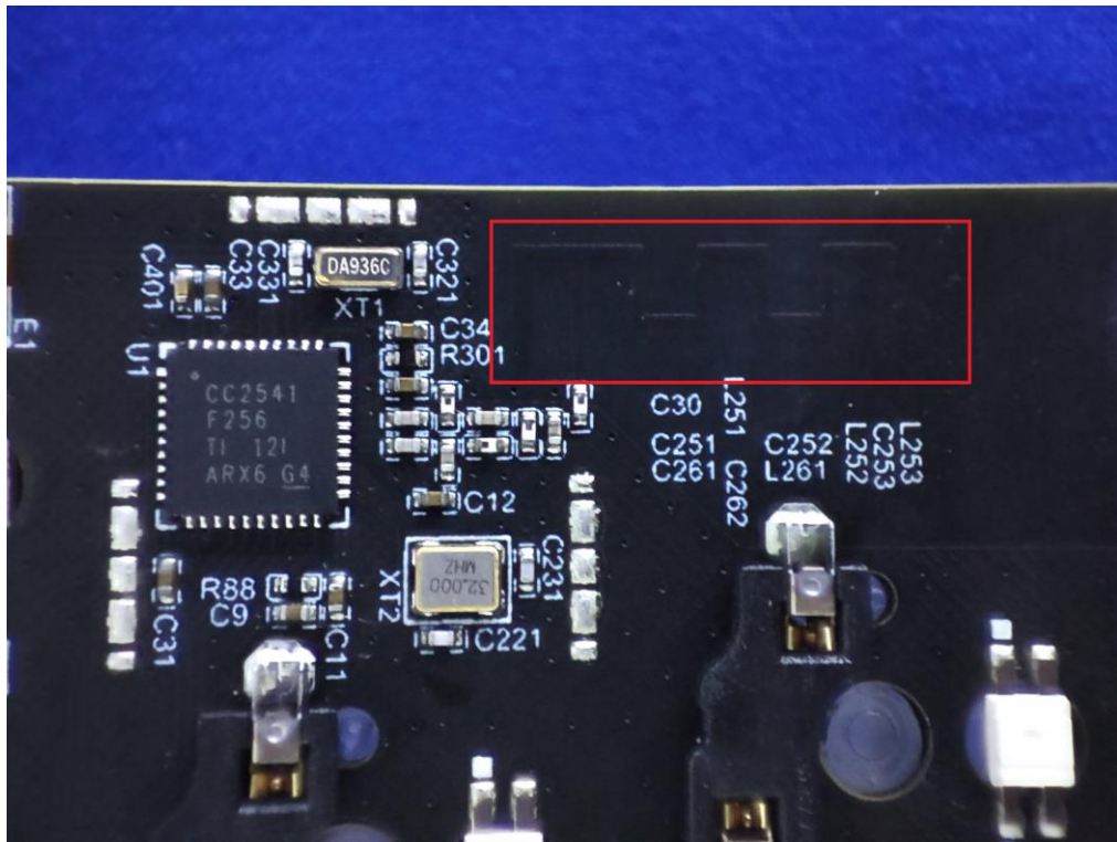
Photo 6: Internal View for RF Module
