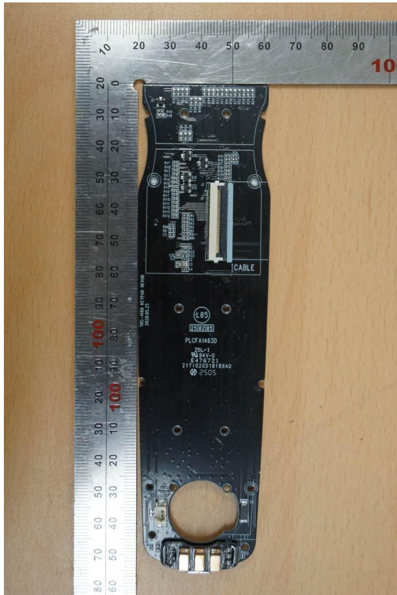
< Down-side board bottom view >
