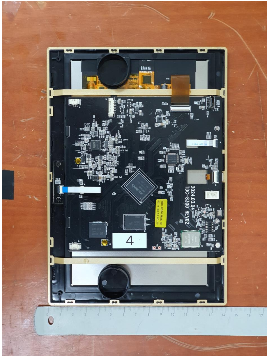
< Inside view #1 >
