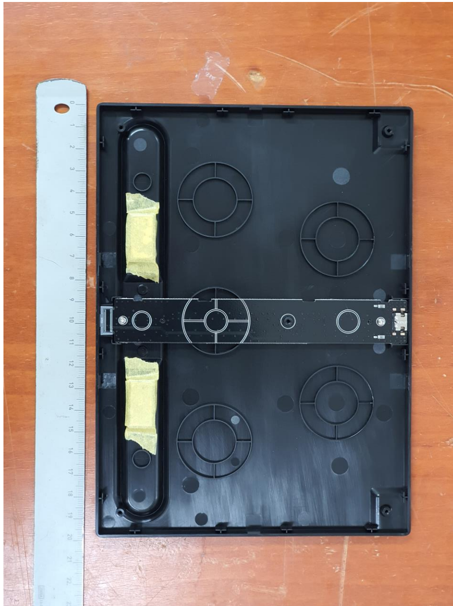
< Charging cradle inside view #2>
