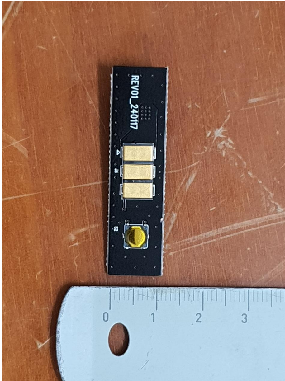
< Charge PCB bottom view >
