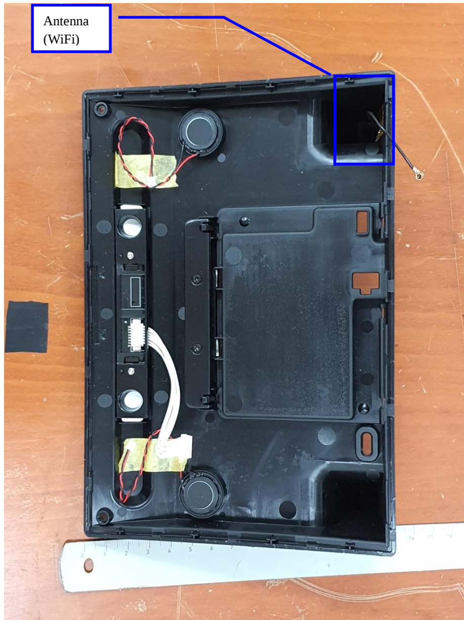
< Inside view #2 >
