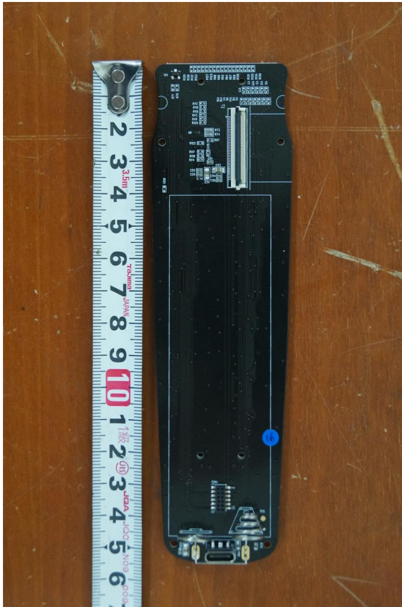
< Sub board Bottom view >
