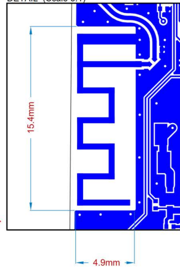
DETAIL (Scale 5:1)
