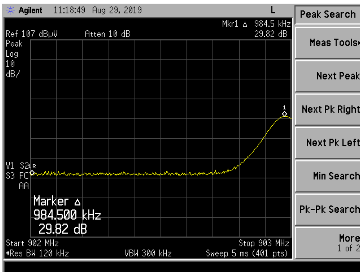
Figure 3. Band Edge Compliance, Low Channel Delta
