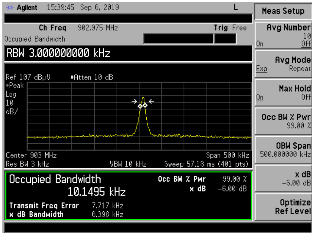
Figure 4. Occupied Bandwidth – Low Channel
