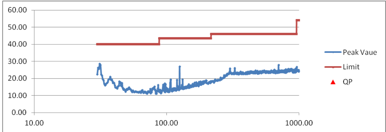
Figure 7. Radiated Emissions 30 MHz - 1000 MHz, Horizontal
