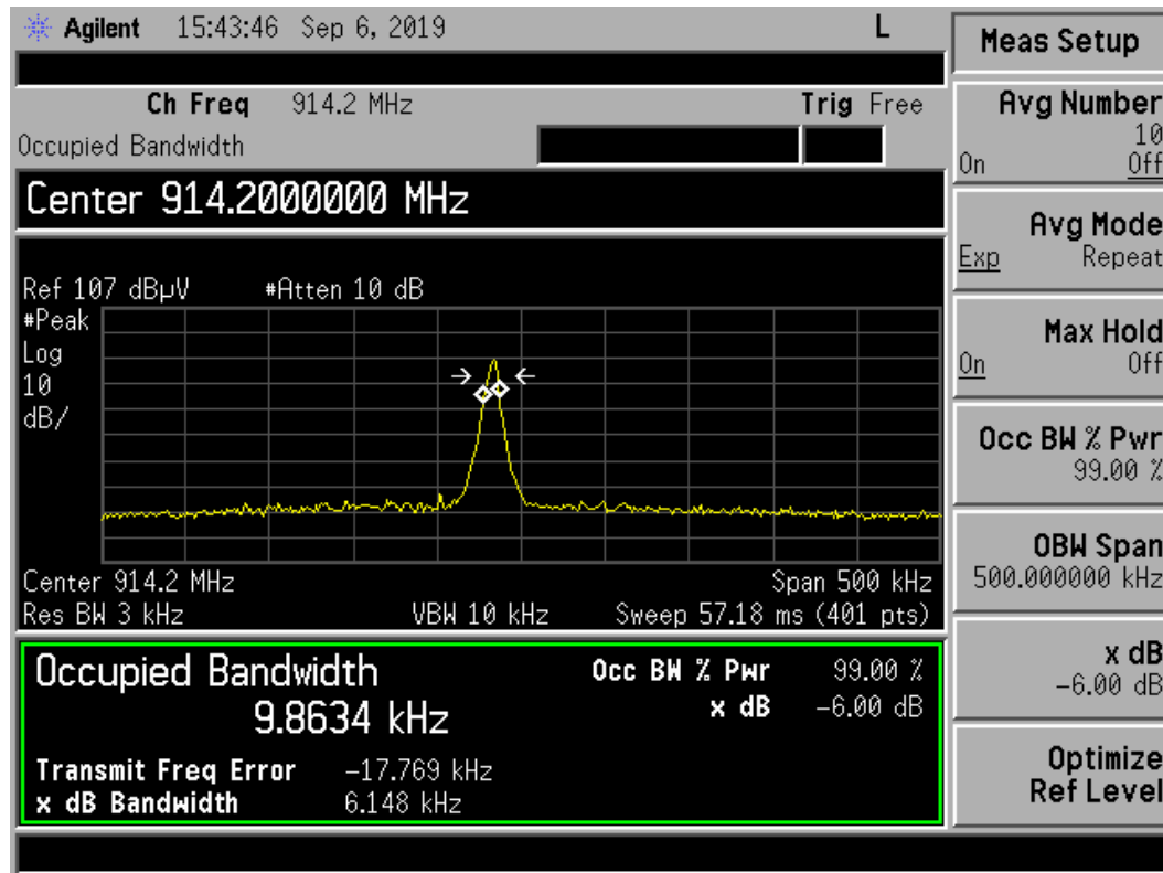
Figure 6. Occupied Bandwidth – High Channel
