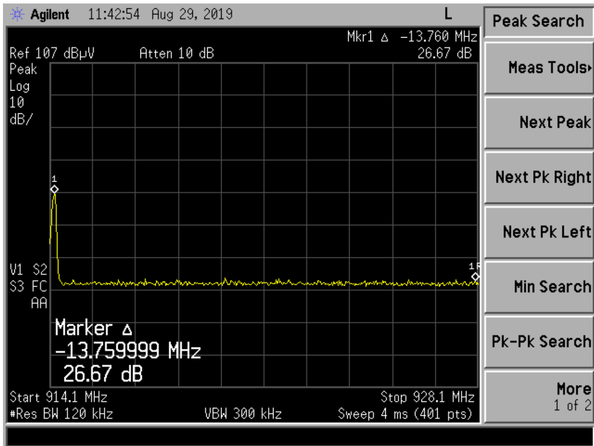
Figure 2. Band Edge Compliance, High Channel Delta
