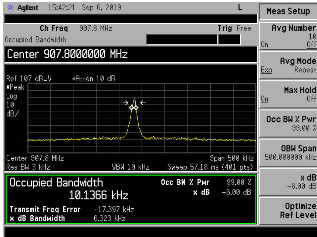
Figure 5. Occupied Bandwidth – Mid Channel
