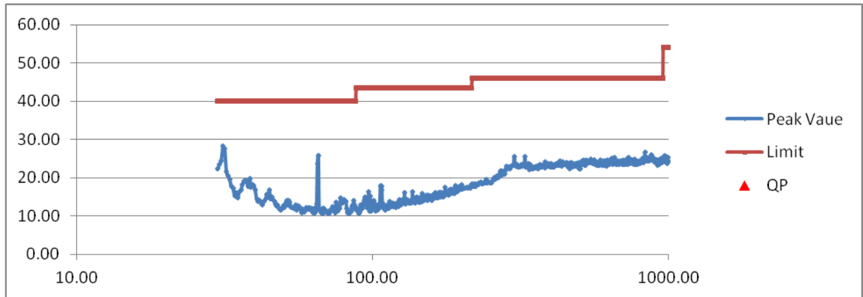
Figure 8. Radiated Emissions 30 MHz - 1000 MHz, Vertical
