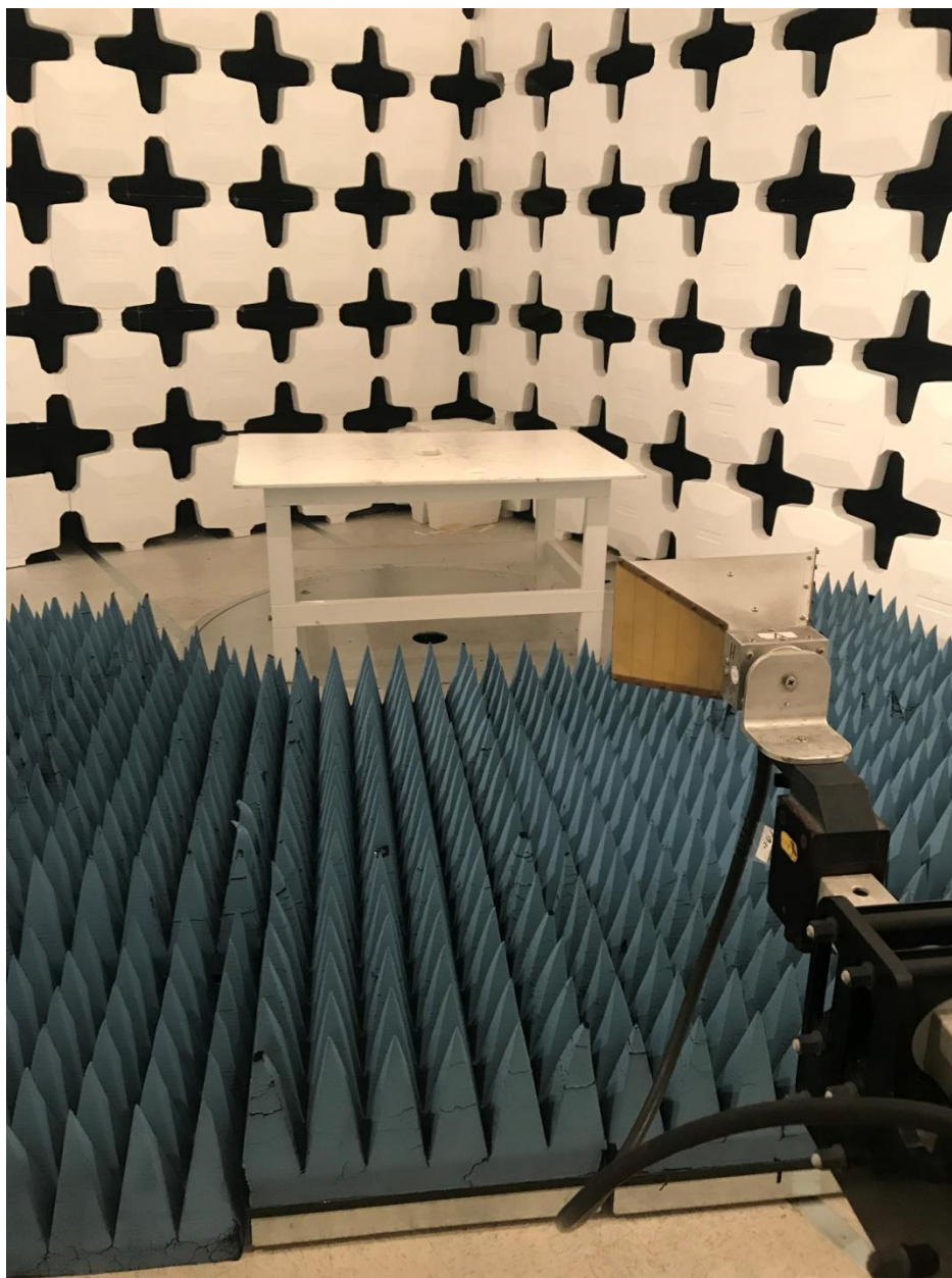
Figure 5. Radiated Emissions, Above 1000 MHz (unintentional emissions)
