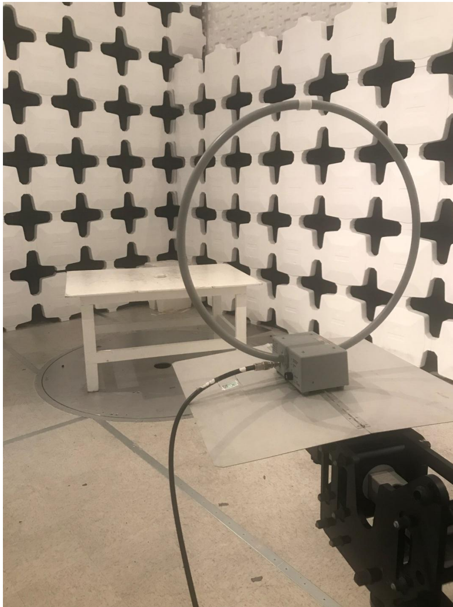
Figure 2. Radiated Emissions, 9 kHz – 30 MHz
