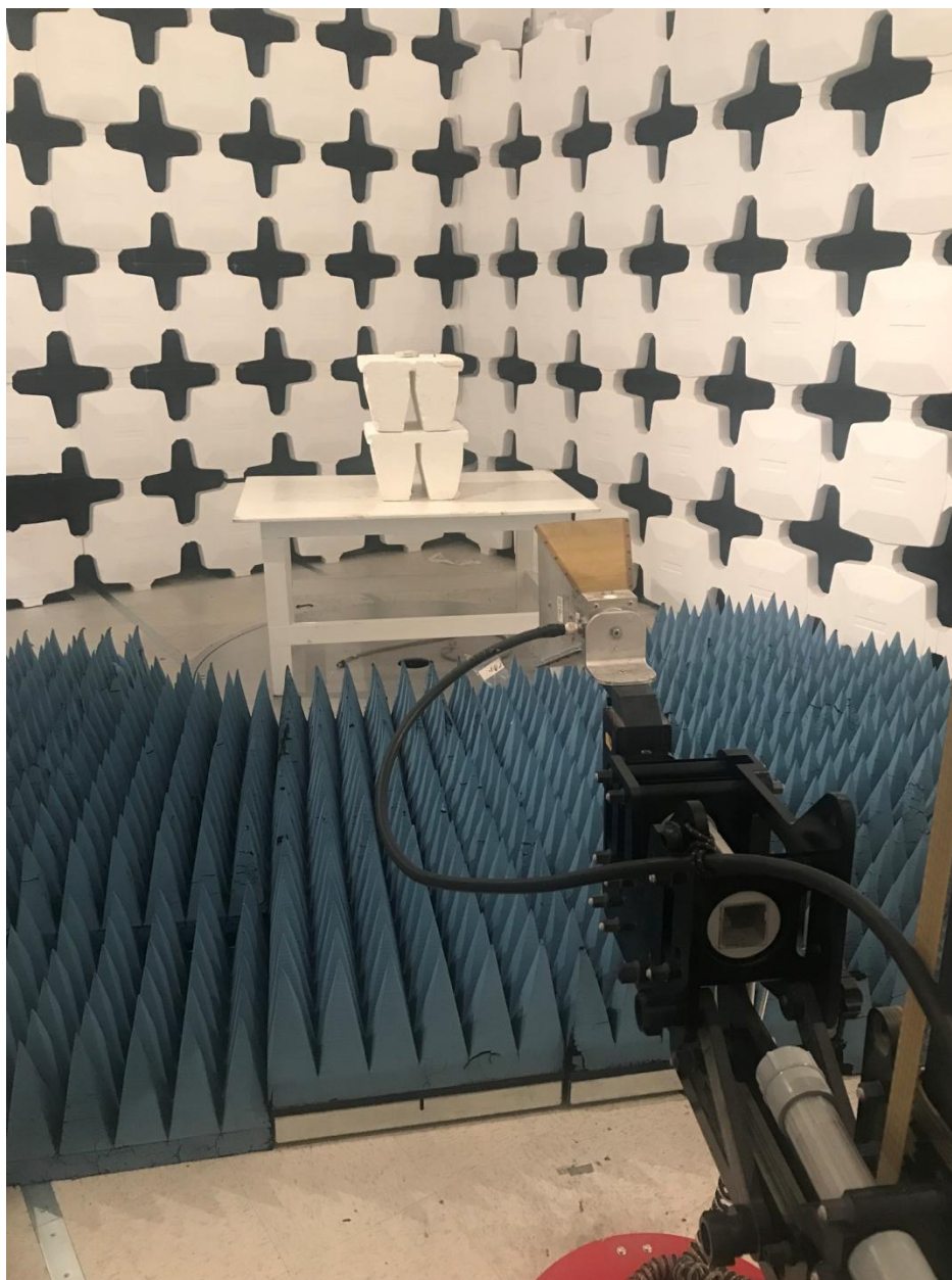
Figure 7. Radiated Emissions Test Setup above 1 GHz (intentional emissions)
