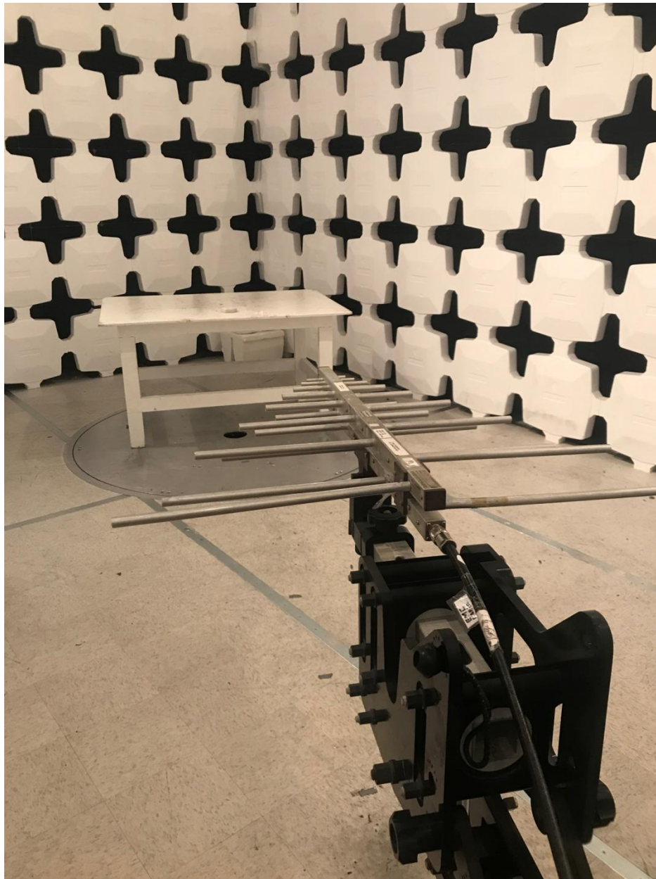
Figure 4. Radiated Emissions, 200 MHz - 1000 MHz
