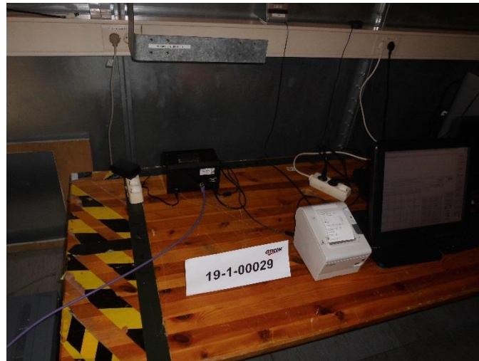
Photograph 1: Mains conducted emission measurements test set-up for measurement of frequency up to 30MHz
