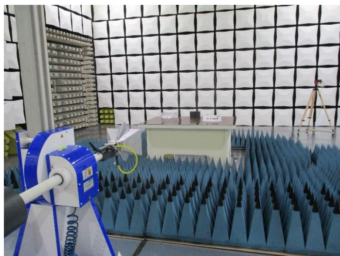
Photograph 3: Radiated emission measurements test set-up for measurement of frequency up to 7 GHz Front side view
