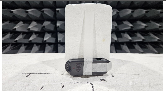
Fig B3 Test Configuration Position at 0 degrees Orientation O2 (Side)
