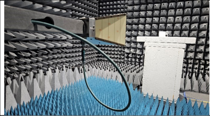
Fig B1 Test Configuration
