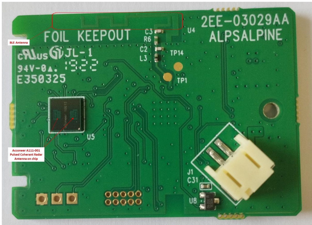
Figure 3: Skoll PCB Side-1 Antennas
