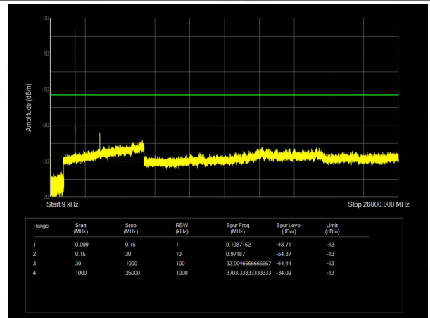
Band25 QAM16 BW=3MHz Channel=26055 RB Size=15 Position=#0
