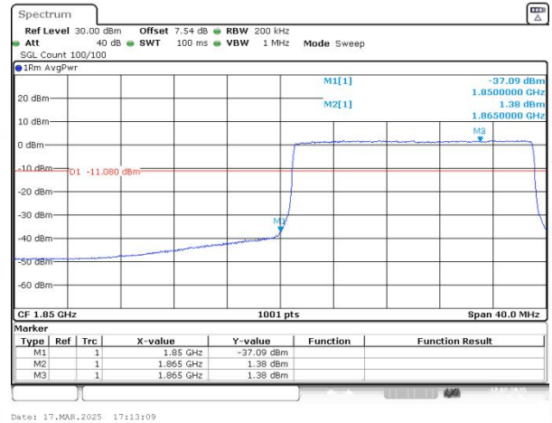
Band25 QAM16 BW=20MHz Channel=26140 RB Size=100 Position=#0
