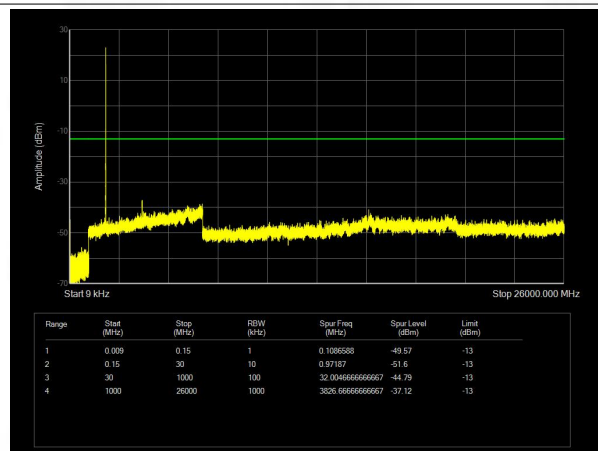
Band25 QAM16 BW=5MHz Channel=26665 RB Size=25 Position=#0
