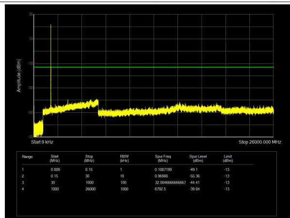
Band25 QAM16 BW=10MHz Channel=26090 RB Size=50 Position=#0
