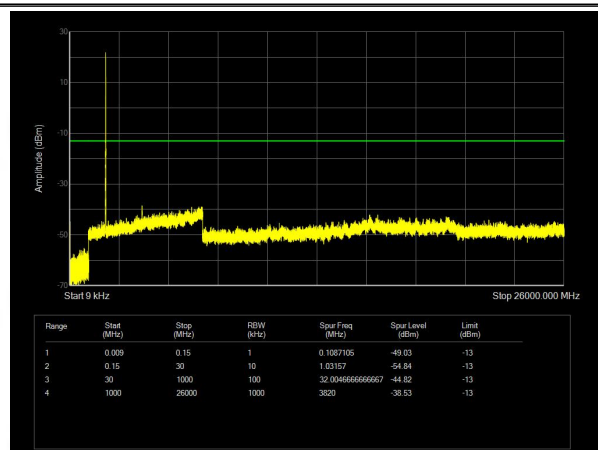
Band25 QAM16 BW=10MHz Channel=26640 RB Size=50 Position=#0
