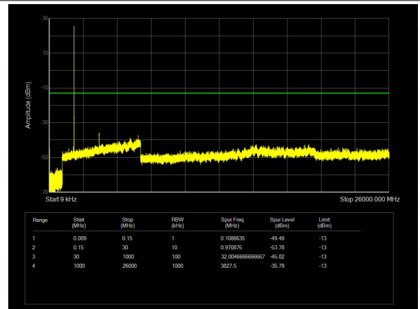
Band25 QAM16 BW=3MHz Channel=26675 RB Size=15 Position=#0
