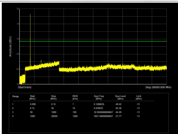
Band25 QPSK BW=5MHz Channel=26665 RB Size=25 Position=#0
