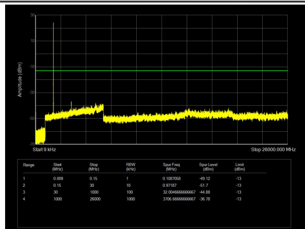
Band25 QAM16 BW=5MHz Channel=26065 RB Size=25 Position=#0
