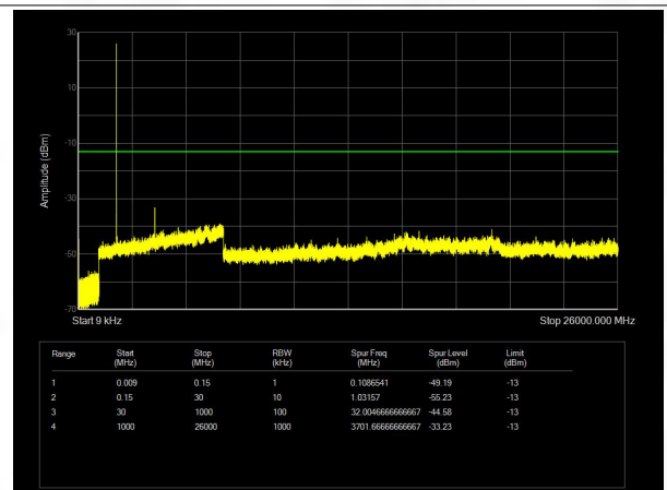
Band25 QAM16 BW=1.4MHz Channel=26047 RB Size=6 Position=#0
