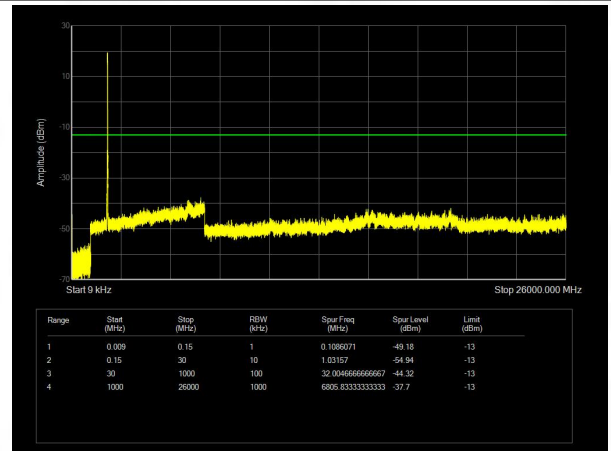
Band25 QAM16 BW=20MHz Channel=26590 RB Size=100 Position=#0
