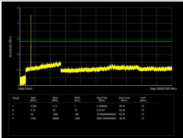
Band25 QPSK BW=20MHz Channel=26590 RB Size=100 Position=#0
