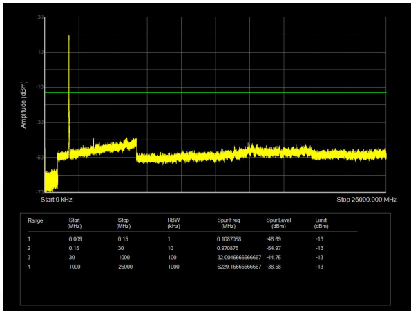
Band25 QPSK BW=20MHz Channel=26140 RB Size=100 Position=#0
