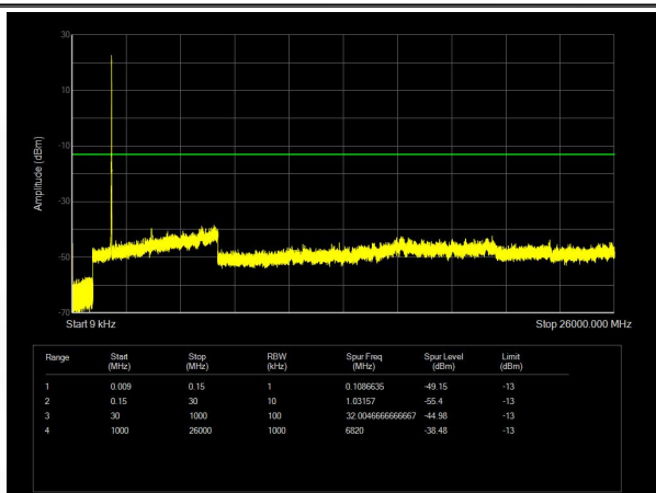
Band25 QPSK BW=10MHz Channel=26640 RB Size=50 Position=#0
