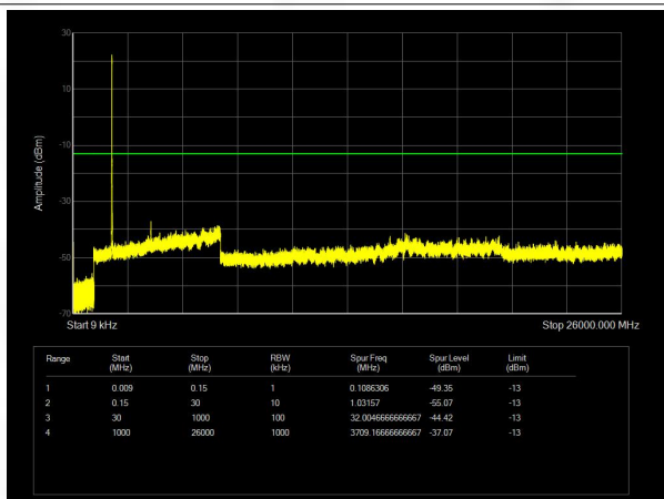
Band25 QPSK BW=10MHz Channel=26090 RB Size=50 Position=#0
