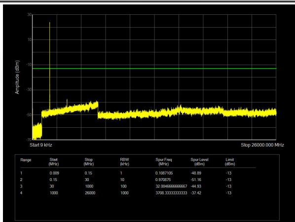
Band25 QPSK BW=5MHz Channel=26065 RB Size=25 Position=#0
