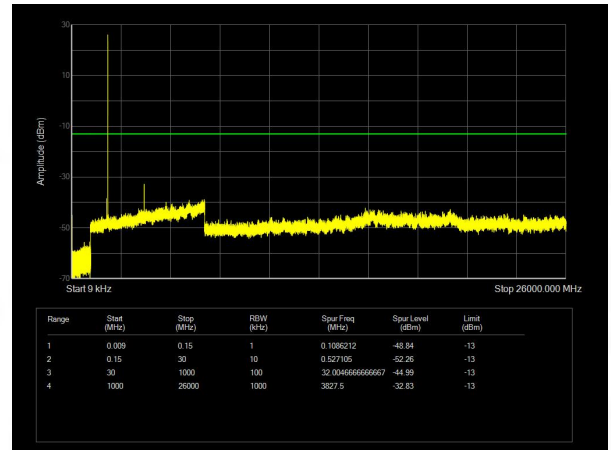
Band25 QAM16 BW=1.4MHz Channel=26683 RB Size=6 Position=#0
