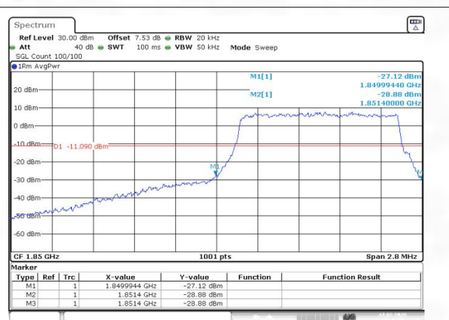
Band25 QAM16 BW=1.4MHz Channel=26047 RB Size=6 Position=#0
