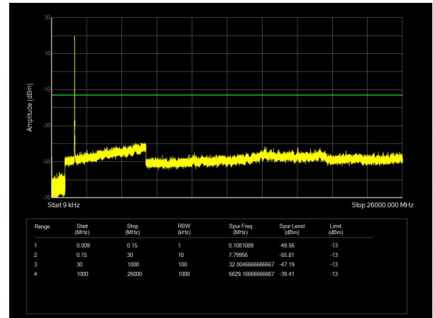
Band4 QPSK BW=15MHz Channel=20025 RB Size=75 Position=#0
