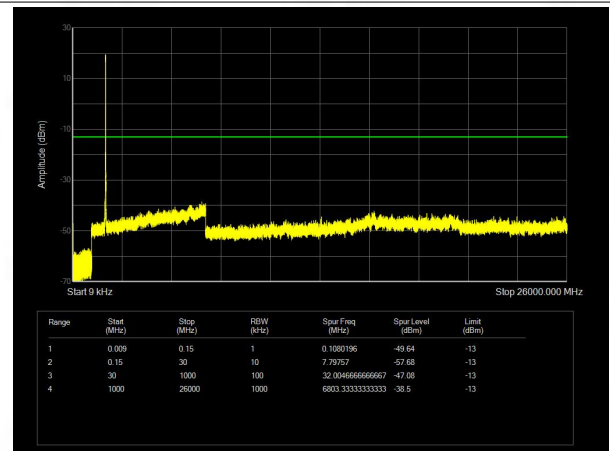
Band4 QPSK BW=15MHz Channel=20325 RB Size=75 Position=#0
