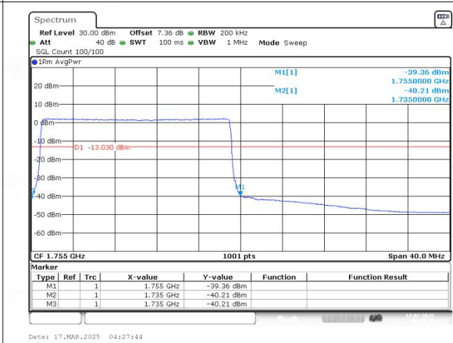
Band4 QAM16 BW=20MHz Channel=20300 RB Size=100 Position=#0
