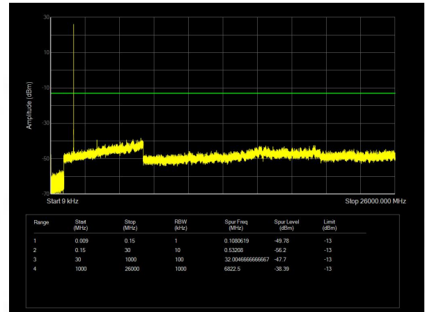
Band4 QAM16 BW=1.4MHz Channel=20393 RB Size=6 Position=#0
