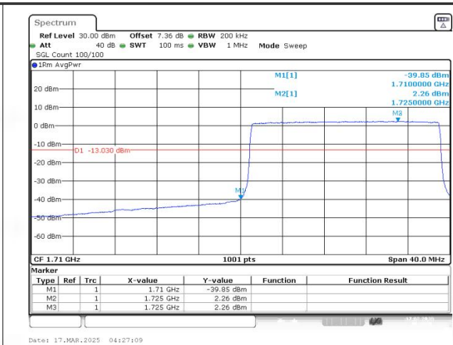
Band4 QAM16 BW=20MHz Channel=20050 RB Size=100 Position=#0
