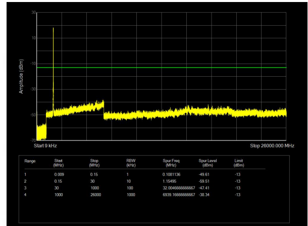
Band4 QPSK BW=20MHz Channel=20300 RB Size=100 Position=#0
