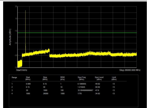
Band4 QAM16 BW=3MHz Channel=20385 RB Size=15 Position=#0
