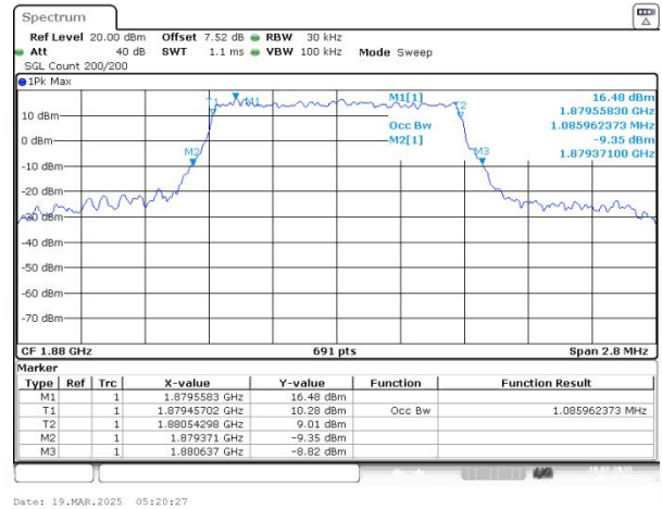
Band2 QAM16 BW=1.4MHz Channel=18900 RB Size=6 Position=#0
