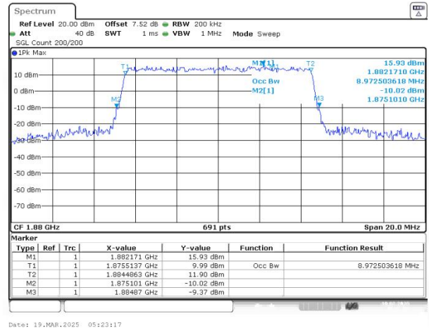
Band2 QAM16 BW=10MHz Channel=18900 RB Size=50 Position=#0
