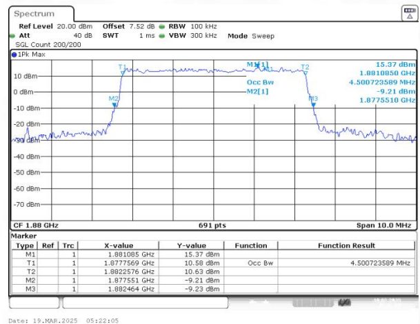
Band2 QAM16 BW=5MHz Channel=18900 RB Size=25 Position=#0
