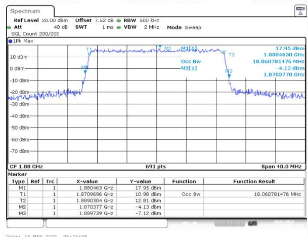
Band2 QAM16 BW=20MHz Channel=18900 RB Size=100 Position=#0
