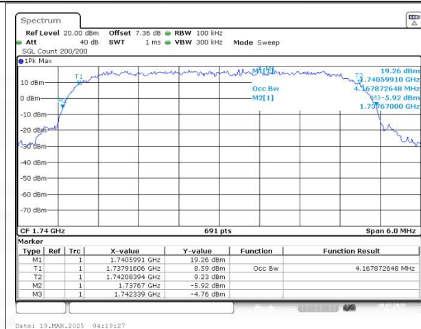
WCDMA Band4 Channel=1450
