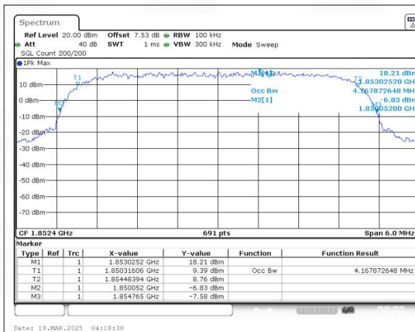
WCDMA Band2 Channel=9262
