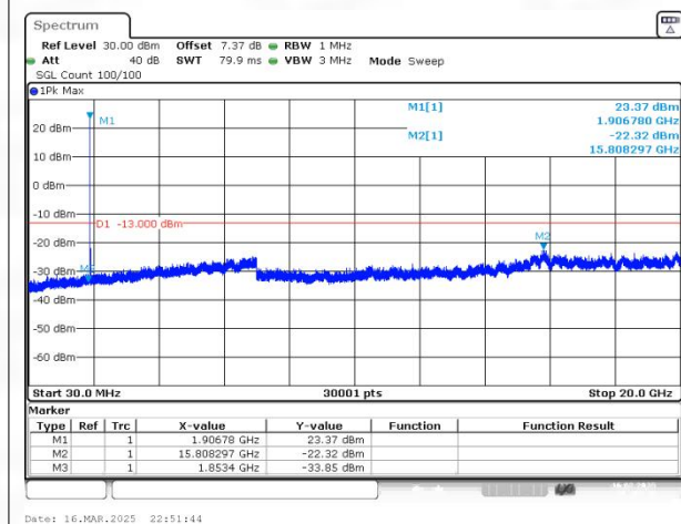
WCDMA Band2 Channel=9538
