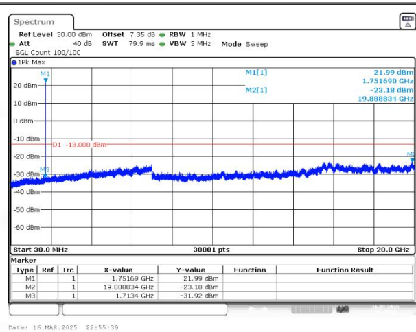
WCDMA Band4 Channel=1513
