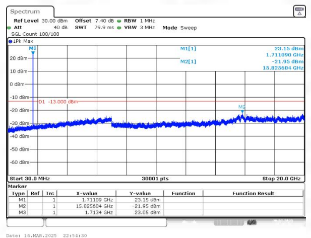
WCDMA Band4 Channel=1312
