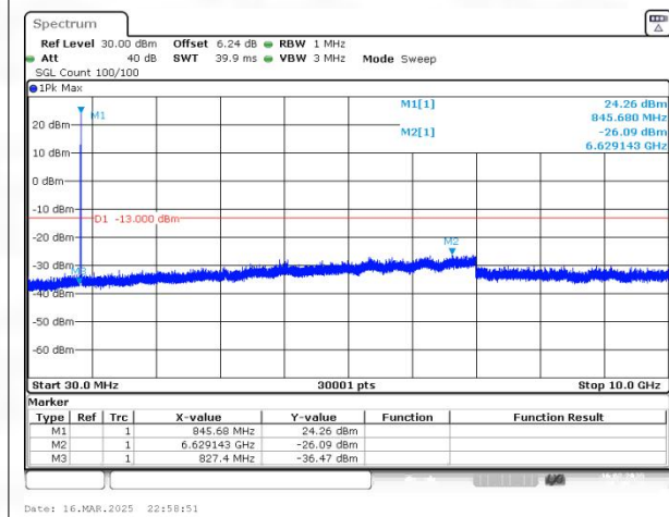
WCDMA Band5 Channel=4233
