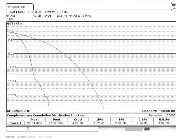
WCDMA Band2 Channel=9538
