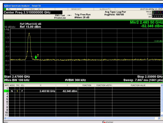
Out Of Band Emission 8DPSK_3-DH3_Channel 78
