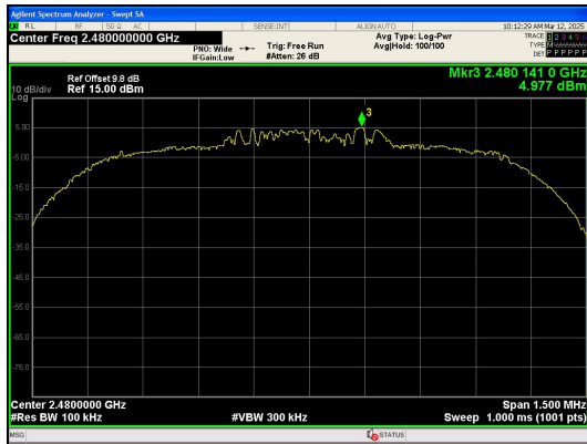
In-Band Reference Level \pi/4 DQPSK_2-DH3_Channel 78
