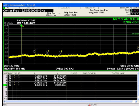
30.0 MHz - 25000.0 MHz 8DPSK_3-DH3_Channel 39
