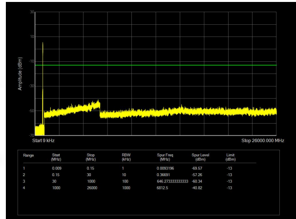
Band5 QAM16 BW=10MHz Channel=20600 RB Size=50 Position=#0
