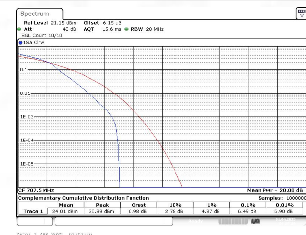
Band12 QAM16 BW=3MHz Channel=23095 RB Size=1 Position=#0
