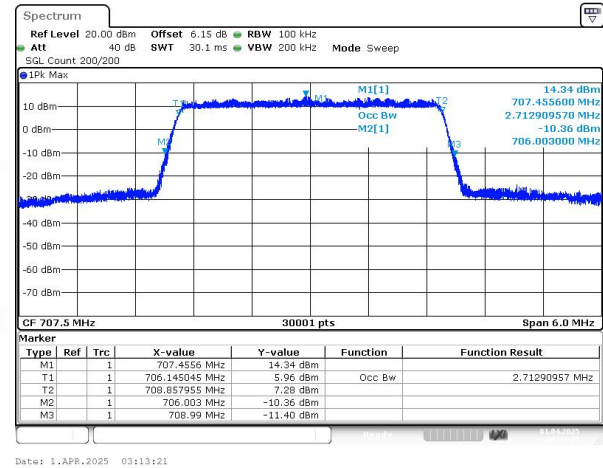
Band12 QAM16 BW=3MHz Channel=23095 RB Size=15 Position=#0
