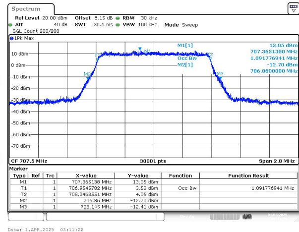
Band12 QAM16 BW=1.4MHz Channel=23095 RB Size=6 Position=#0
