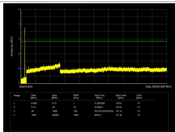
Band12 QAM16 BW=10MHz Channel=23060 RB Size=50 Position=#0
