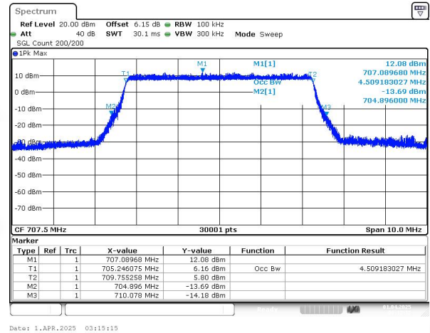
Band12 QAM16 BW=5MHz Channel=23095 RB Size=25 Position=#0
