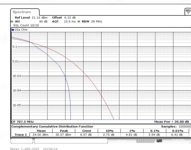
Band12 QAM16 BW=1.4MHz Channel=23095 RB Size=1 Position=#0
