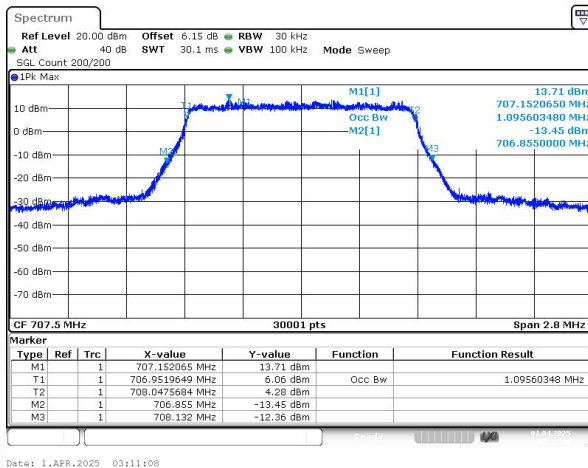
Band12 QPSK BW=1.4MHz Channel=23095 RB Size=6 Position=#0
