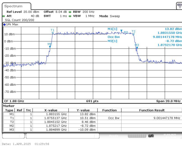
Band2 QPSK BW=10MHz Channel=18900 RB Size=50 Position=#0
