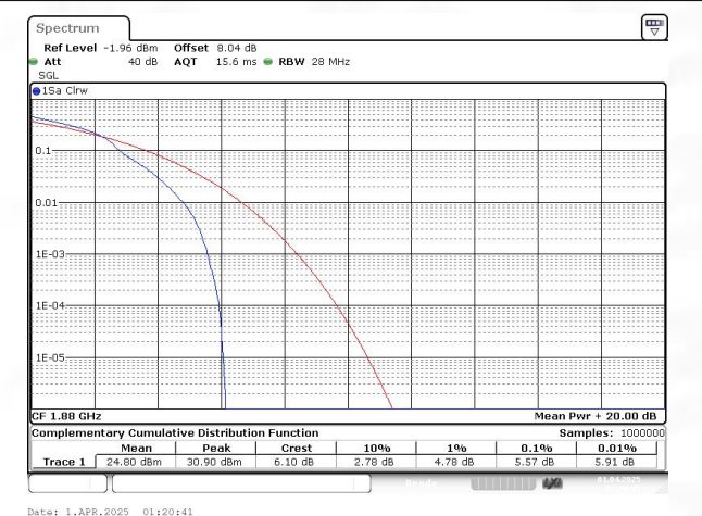
Band2 QAM16 BW=3MHz Channel=18900 RB Size=1 Position=#0
