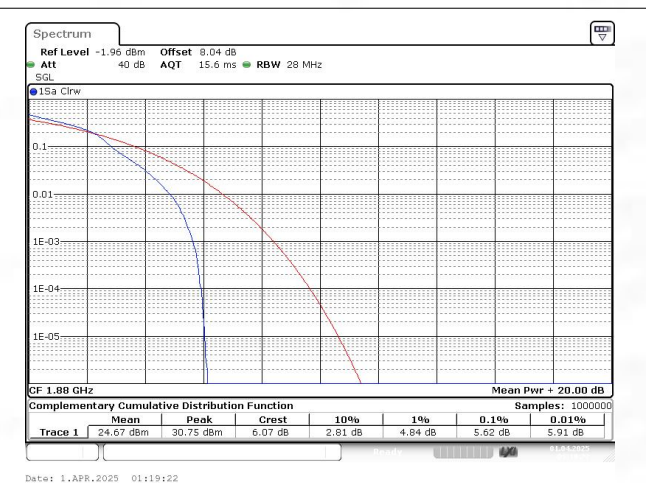
Band2 QAM16 BW=1.4MHz Channel=18900 RB Size=1 Position=#0
