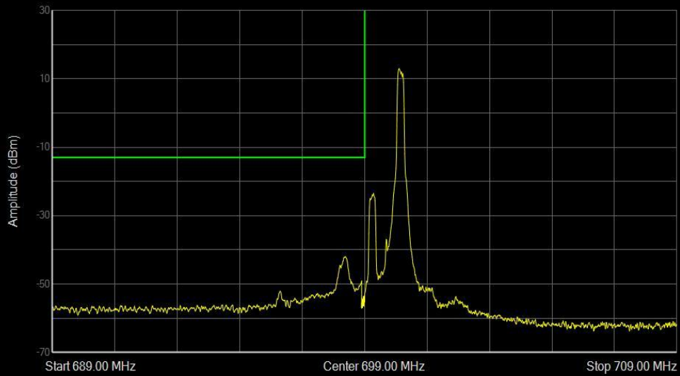
Band12 QAM16 BW=1.4MHz Channel=23017 RB Size=1 Position=#Max
