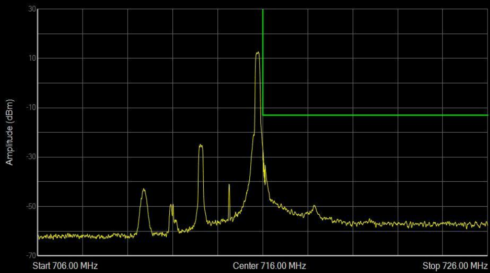
Band12 QAM16 BW=3MHz Channel=23165 RB Size=1 Position=#Max
