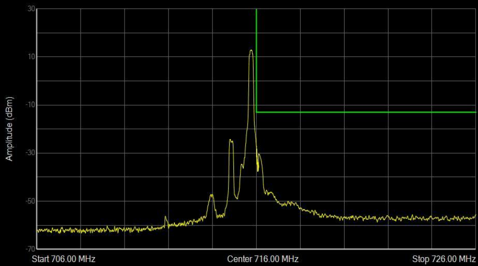
Band12 QAM16 BW=1.4MHz Channel=23173 RB Size=1 Position=#Max
