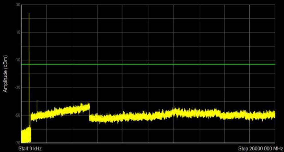
Band26(814-824) QAM16 BW=5MHz Channel=26740 RB Size=1 Position=#0
