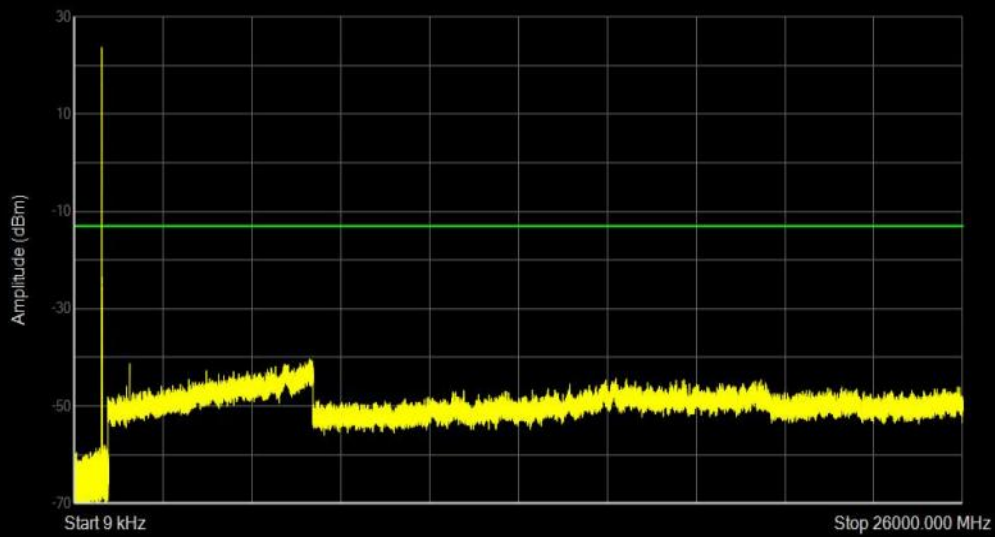
Band26(814-824) QAM16 BW=1.4MHz Channel=26740 RB Size=1 Position=#0
