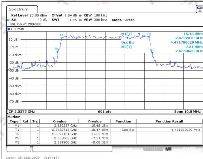
Band41(2555-2655) QPSK BW=5MHz Channel=40265 RB Size=25 Position=#0
