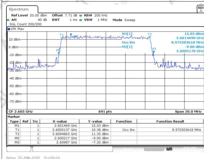
Band41(2555-2655) QPSK BW=10MHz Channel=40740 RB Size=50 Position=#0
