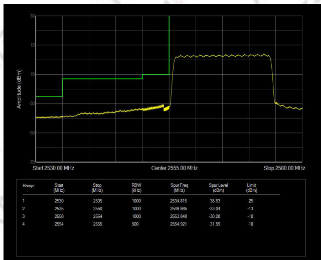
Band41(2555-2655) QPSK BW=20MHz Channel=40340 RB Size=100 Position=#0
