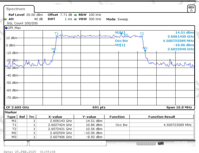
Band41(2555-2655) QPSK BW=5MHz Channel=40740 RB Size=25 Position=#0
