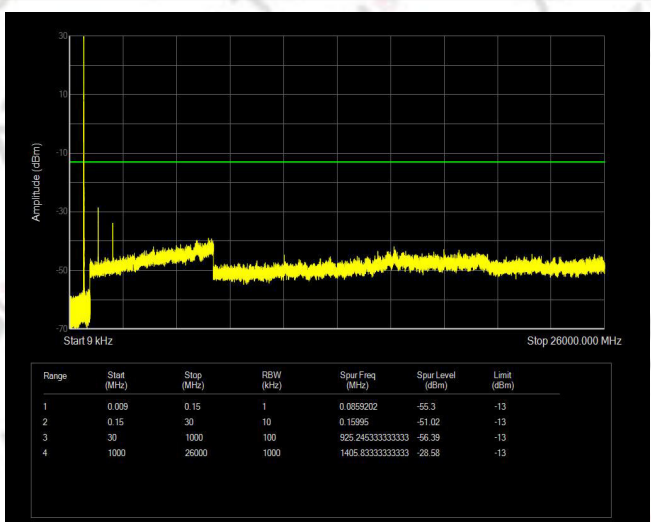
Band12 QPSK BW=10MHz Channel=23095
