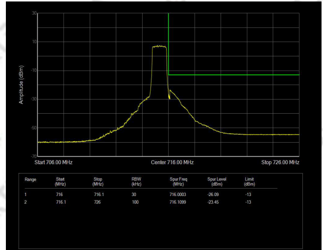
Band12 QAM16 BW=1.4MHz Channel=23173 RB Size=6 Position=#0
