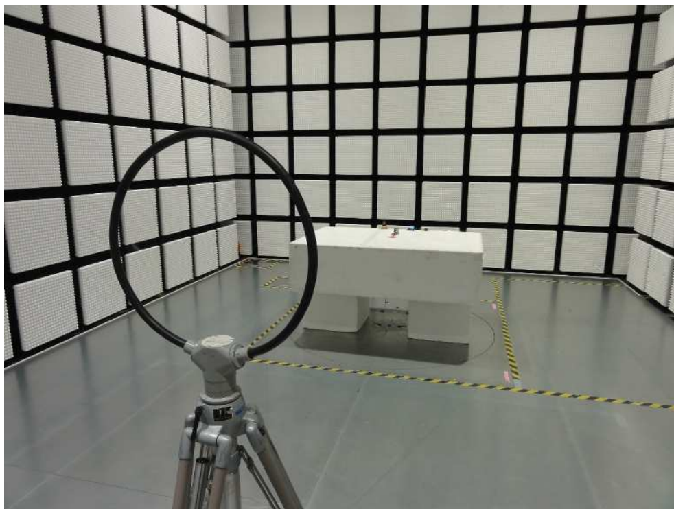
– Overview (9 kHz – 30 MHz Horizontal) –
