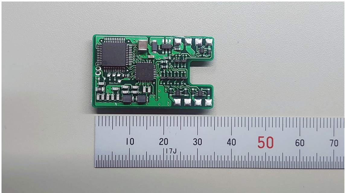
- Rear View-
