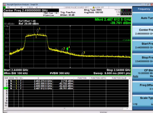
Right bandedge
