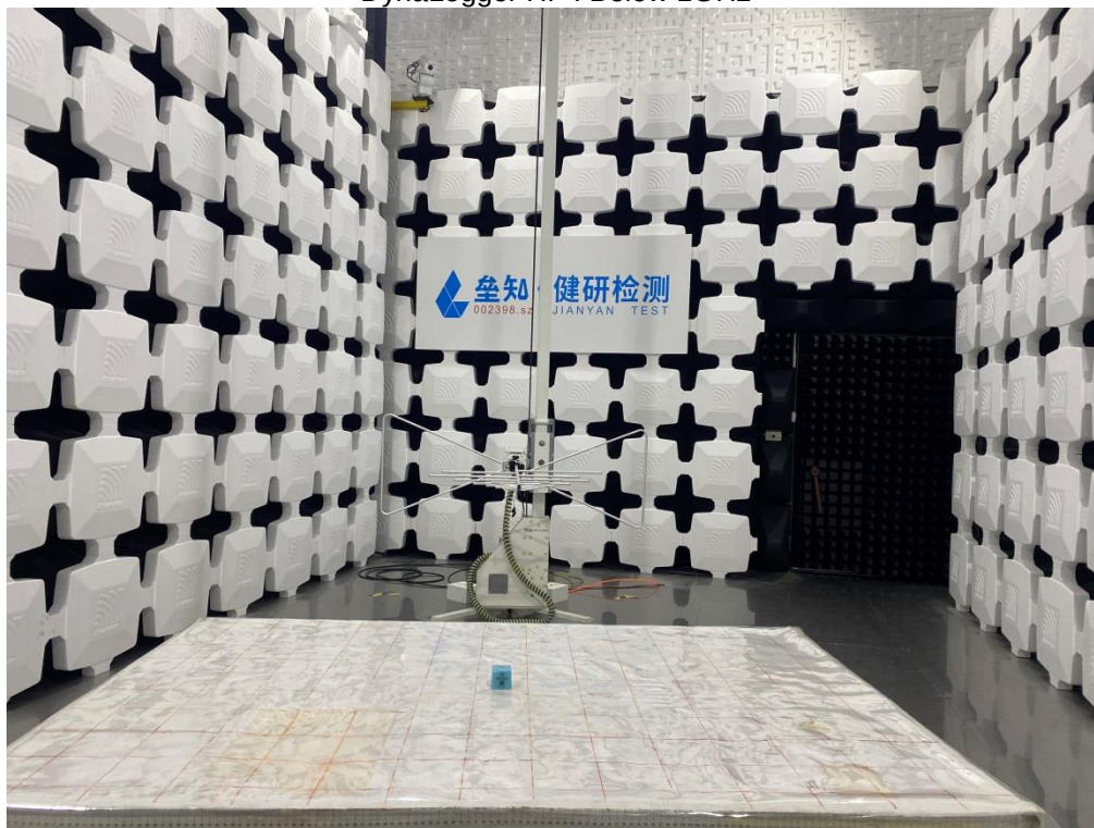
Radiated Emission DynaLogger HF : Below 1GHz
