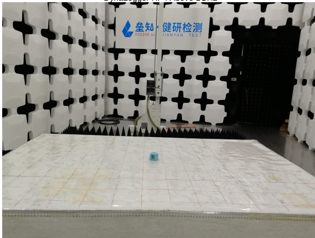
Radiated Emission DynaLogger HF : Above 1GHz
