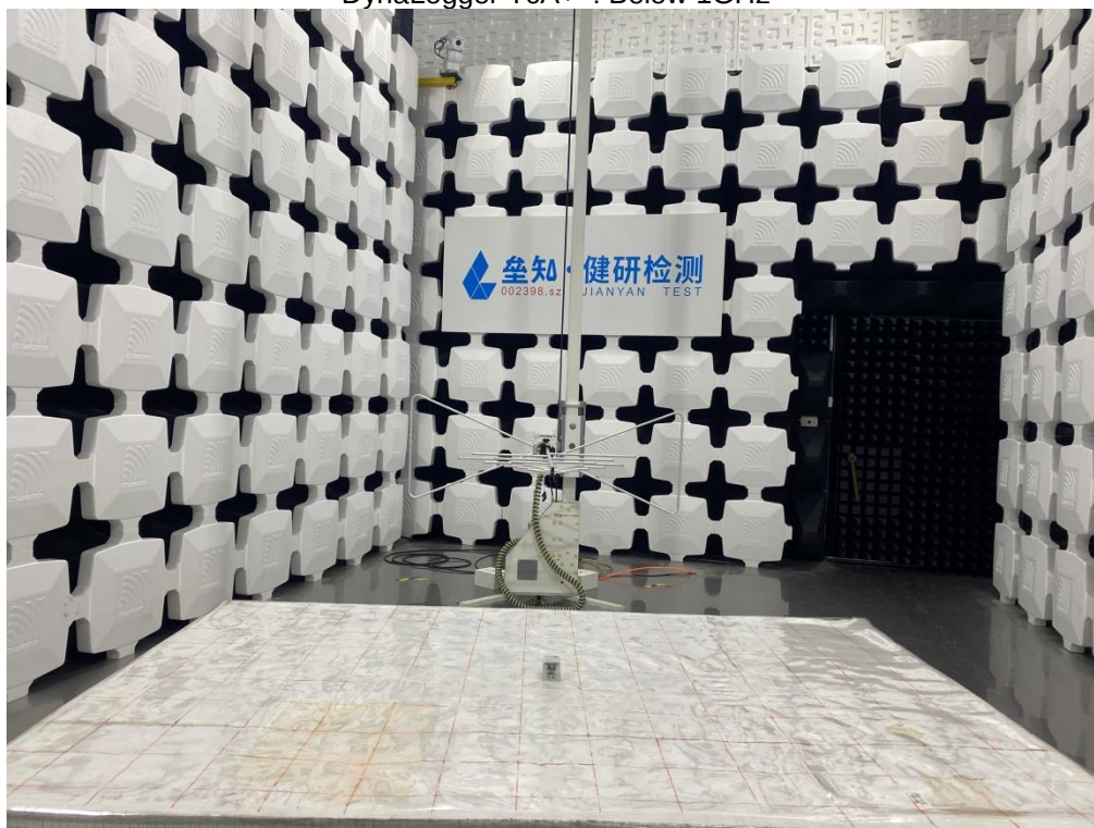
DynaLogger TcA+ : Below 1GHz
