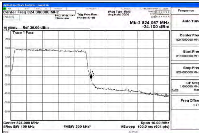
Band Edge Test Graph(s) (Channel Bandwidth: 5 MHz)_HCH_16QAM
