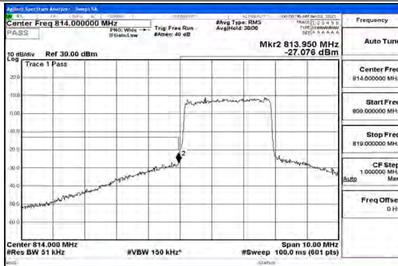
Band Edge Test Graph(s) (Channel Bandwidth: 5 MHz)_LCH_16QAM
