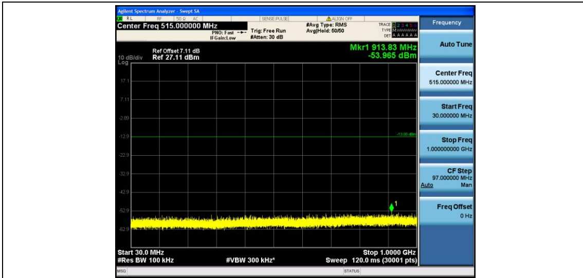
Band2-1.4MHz-QPSK-18607-1RB#0-30~1000MHz
