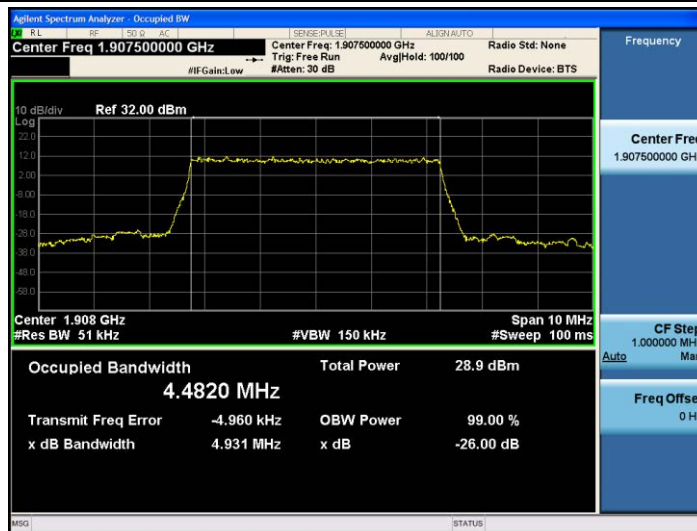
Band2-5MHz-QPSK-19175-25RB#0-4.4820
