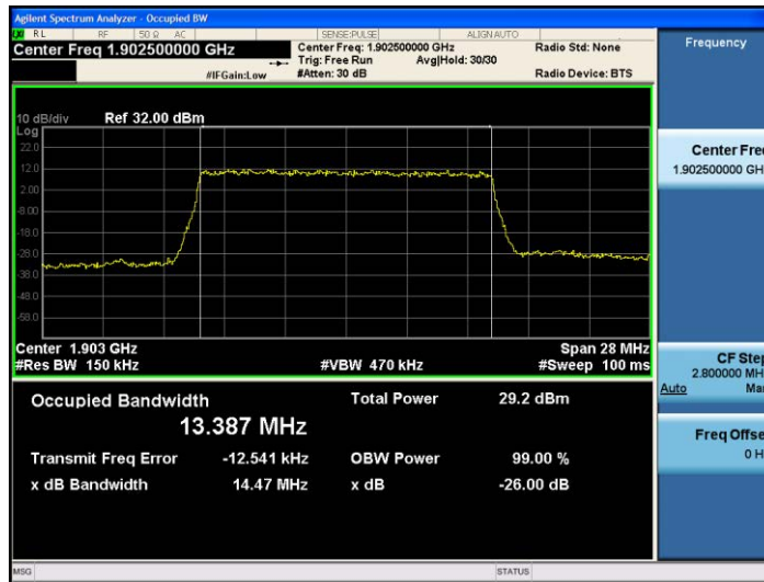
Band2-15MHz-QPSK-19125-75RB#0-13.387
