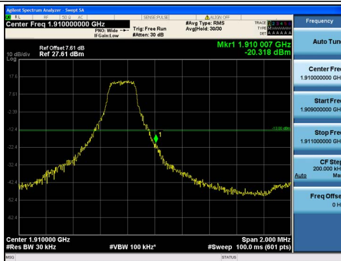
Band2-3MHz-16QAM-19185-1RB#14
