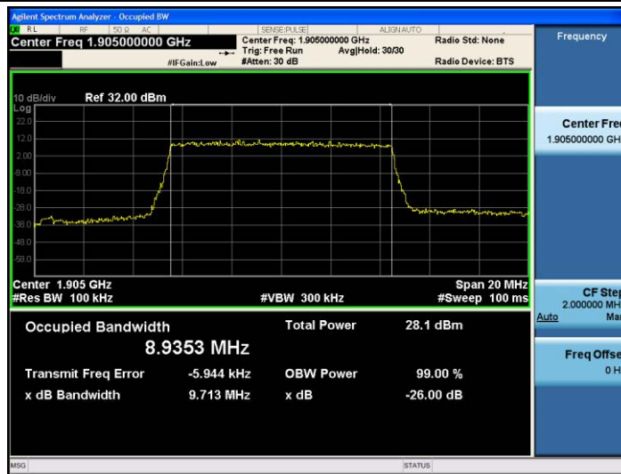
Band2-10MHz-16QAM-19150-50RB#0-8.9353
