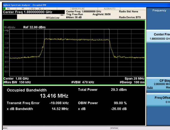
Band2-15MHz-QPSK-18900-75RB#0-13.416
