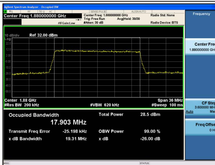
Band2-20MHz-16QAM-18900-100RB#0-17.903
