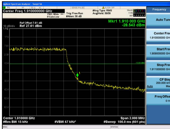
Band2-1.4MHz-16QAM-19193-6RB#0
