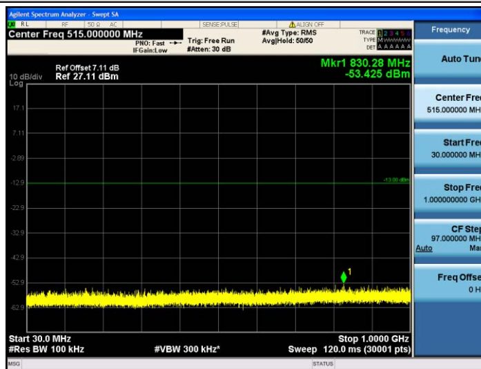
Band2-1.4MHz-16QAM-18900-1RB#0-30~1000MHz
