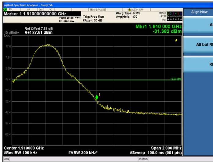
Band2-10MHz-16QAM-19150-1RB#49
