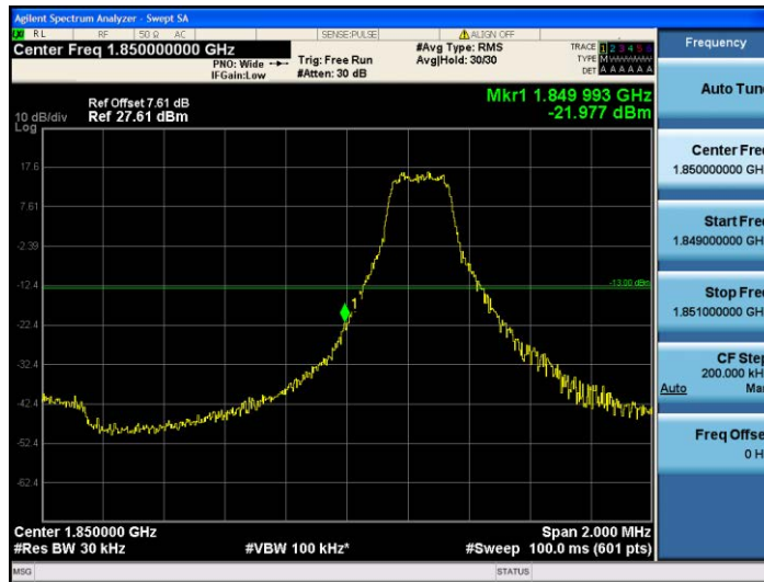
Band2-3MHz-16QAM-18615-1RB#0
