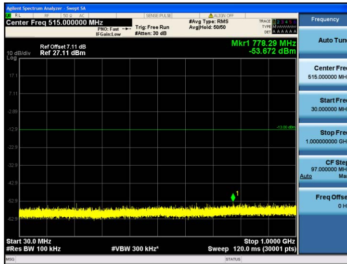
Band2-1.4MHz-16QAM-18607-1RB#0-30~1000MHz
