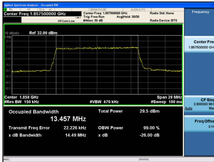
Band2-15MHz-QPSK-18675-75RB#0-13.457
