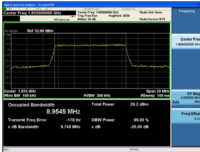
Band2-10MHz-QPSK-18650-50RB#0-8.9545
