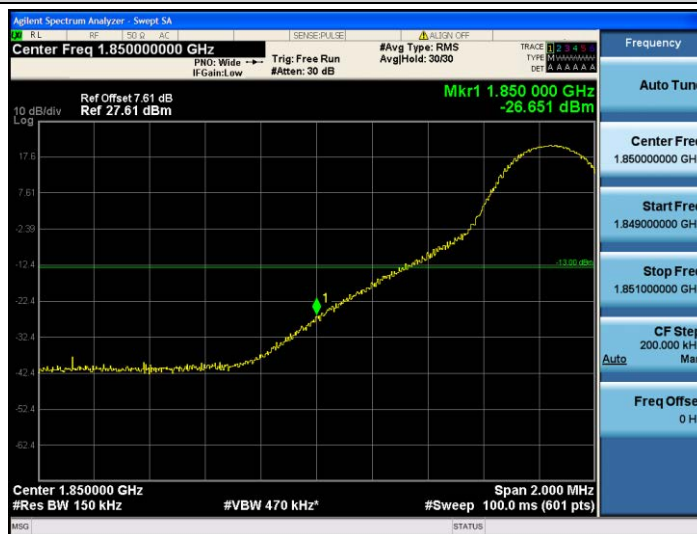
Band2-15MHz-QPSK-18675-1RB#0
