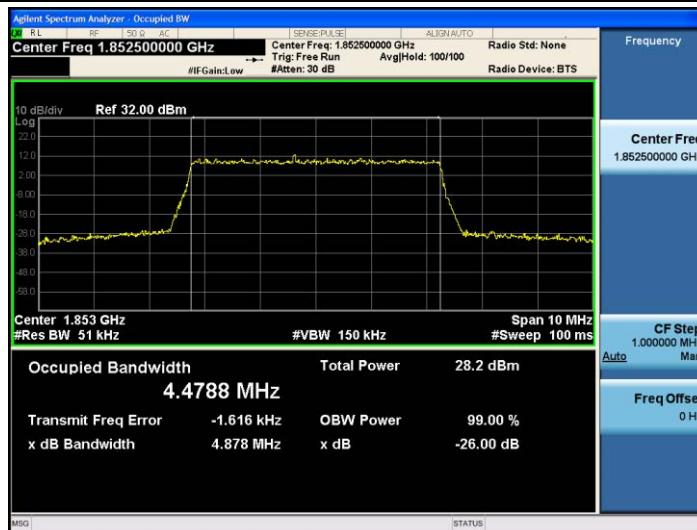
Band2-5MHz-16QAM-18625-25RB#0-4.4788
