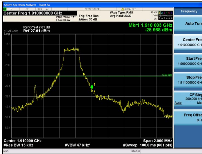
Band2-1.4MHz-16QAM-19193-1RB#5
