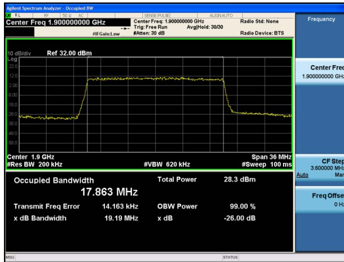
Band2-20MHz-16QAM-19100-100RB#0-17.863
