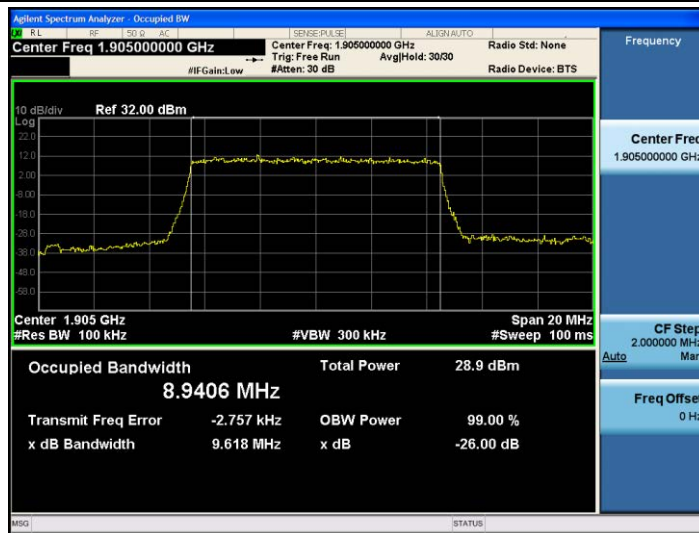
Band2-10MHz-QPSK-19150-50RB#0-8.9406
