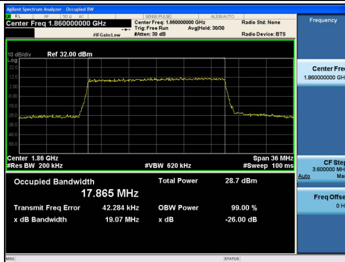
Band2-20MHz-16QAM-18700-100RB#0-17.865
