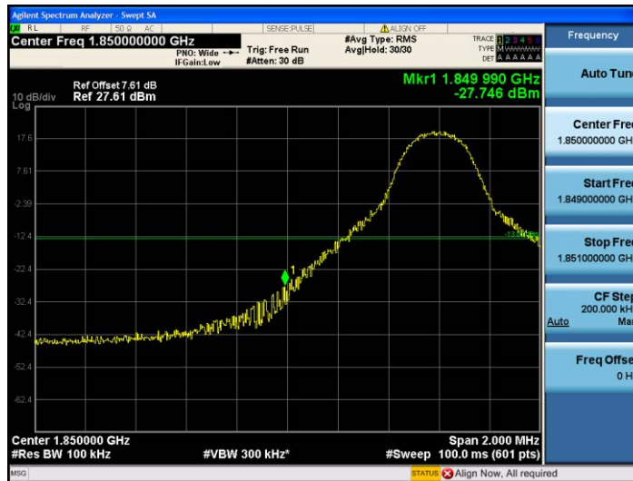
Band2-10MHz-16QAM-18650-1RB#0
