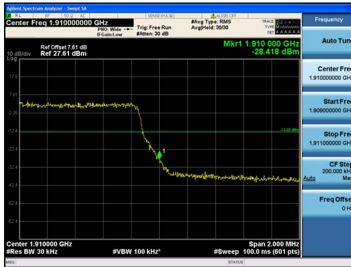
Band2-3MHz-16QAM-19185-15RB#0
