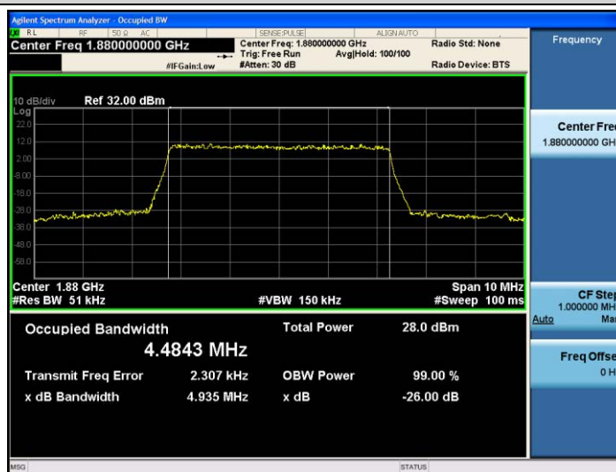
Band2-5MHz-16QAM-18900-25RB#0-4.4843
