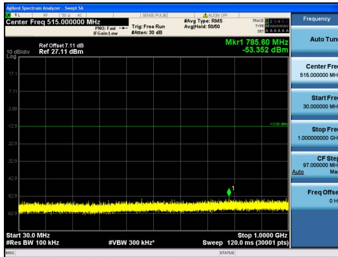
Band2-1.4MHz-16QAM-19193-1RB#0-30~1000MHz
