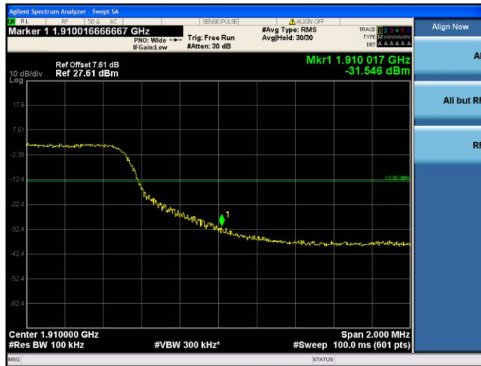
Band2-10MHz-QPSK-19150-50RB#0
