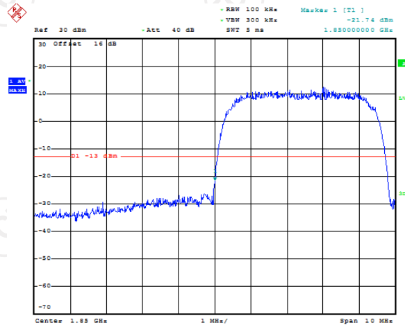
Lower Band Edge Plot on Channel 9262
