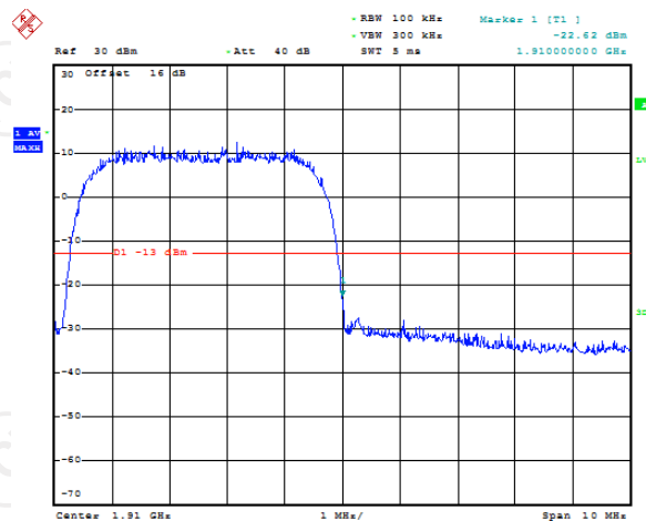
Higher Band Edge Plot on Channel 9538
