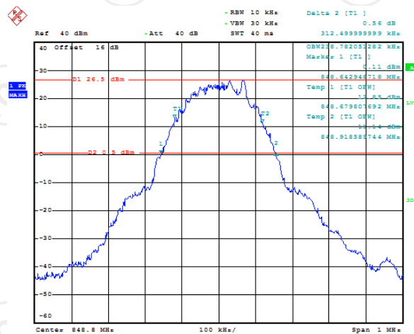
26dB&99% Occupied Bandwidth Plot on Channel 251
